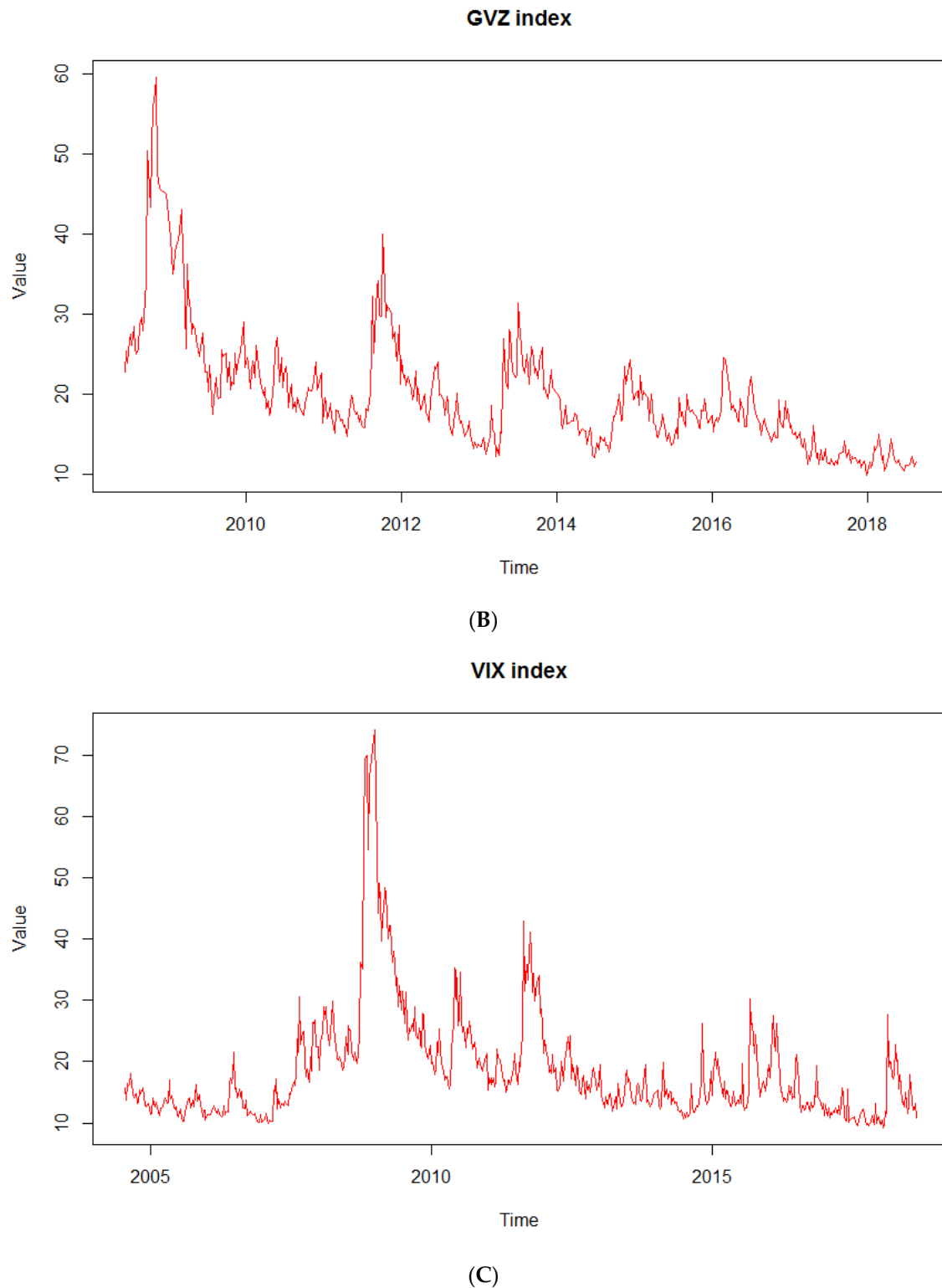
Figure 2. (A) OVX index, 14 May 2007–15 August 2018. Note: This Figure presents the index OVX. (B) GVZ index, 3 June 2008–15 August 2018. Note: This Figure presents the index GVZ. (C) VIX index, 4 July 2004–15 August 2018. Note: This Figure presents the index VIX.
