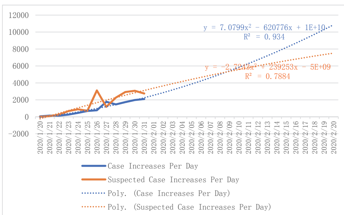
Figure 6. Trend prediction of suspected case increases per day and number of cases increasing per day based on the Excel–Polynomial Method.
