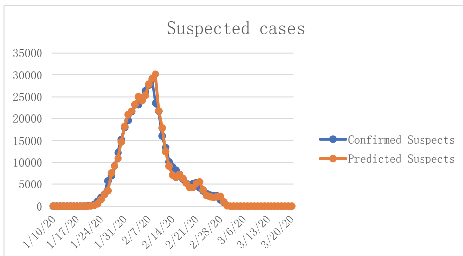
Figure 13. Predicted number of suspects.
