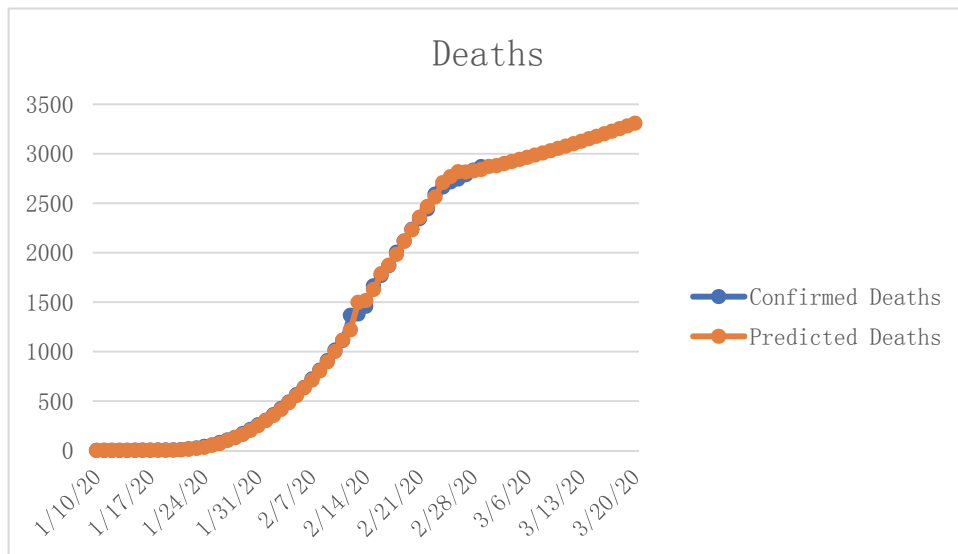
Figure 12. Predicted number of deaths.
