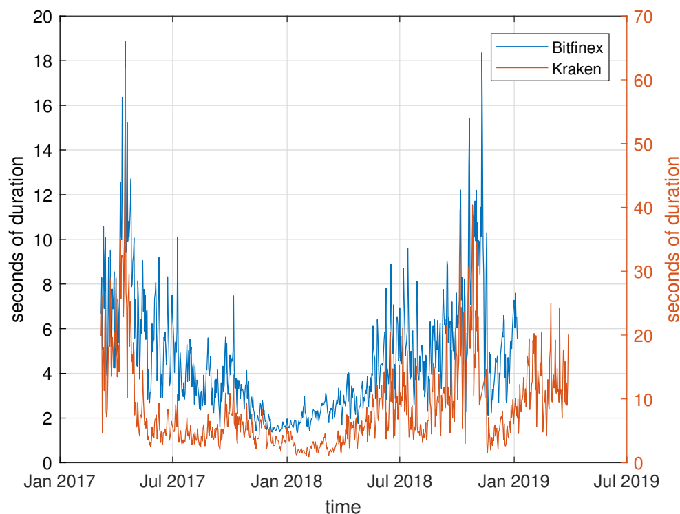
Figure 1. Daily average of raw transaction durations. Note. The figure presents the daily average of raw, unfiltered transaction durations of Bitfinex (blue, left axis) and Kraken (red, right axis) over time.
