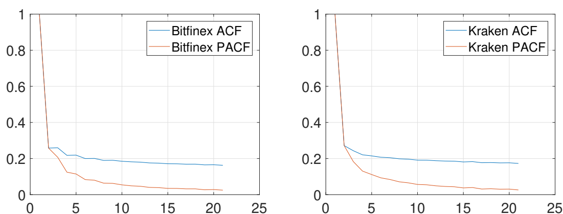
Figure 6. Autocorrelation and Partial Autocorrelation functions. Note. The figure presents the estimated autocorrelation (blue) and partial autocorrelation (red) functions of price durations on Bitfinex (left graph) and Kraken (right graph).
