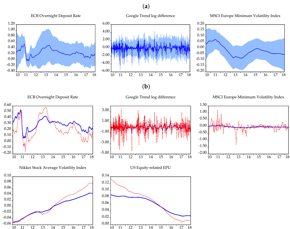
Figure A2. Flexible least squares and state-space varying coefficient paths. (a) Flexible least squares with Kalman filtering varying coefficient paths. (b) Flexible least squares with Kalman filtering (in blue solid lines) and state-space with Kalman filtering (in red dashed lines) varying coefficient paths. Notes: In panel (a) the smoothing parameter has been set to 1; \pm 2 standard deviation bands are in light blue. In panel (b) the smoothing parameter for the FLS has been set to 0.1.
