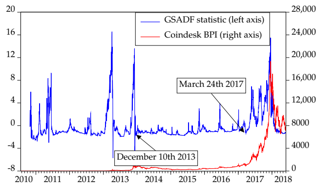
Figure A1. Coindesk BPI and the generalized sup augmented Dickey–Fuller statistic. Notes: The final GSADF statistic is the largest ADF statistic, which in the figure is above 16. The asymptotic 99% critical value for an initial window 5.5% (ours is 3.5%) of the total sample is 2.74 based on numerical simulations with 2000 replications (Phillips et al. 2015). Given that the test statistic exceeds this value in some point (actually multiple) in the sample, there is evidence of bubbly behavior. The corresponding asymptotic critical value for the supremum ADF (SADF) tests constituting the GSADF test is 2.06, providing evidence of multiple cases of bubbles.
