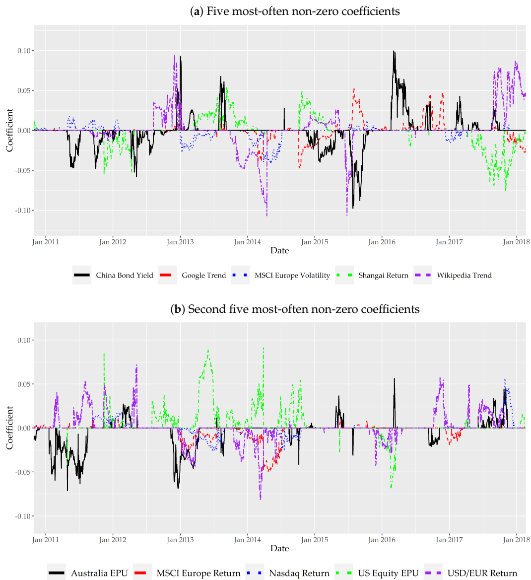
Figure 1. Rolling window PC-LASSO coefficients with market/factor type components. Notes: The window size is 200 observations. All variables are standardized in each window separately. For comparability \lambda = 15 and r = 0.7 across all windows. The ECB the Chinese central bank rates have not been included in the analysis, as they often do not vary within windows. The coefficients on a given date correspond to the window whose 100th observation corresponds to that date. In the first panel are the coefficients of the five independent variables whose coefficients are most often non-zero in the rolling window estimation (for example, the China bond yield is the variable whose coefficient is non-zero the most times; that is, in 994 out of the 2673 rolling window estimations); in the second panel are the five variables with the next highest numbers of non-zero coefficients. Morgan Stanley Capital International’s (MSCI) Europe volatility index and the USD/EUR return have equal numbers of non-zero coefficients (892).
