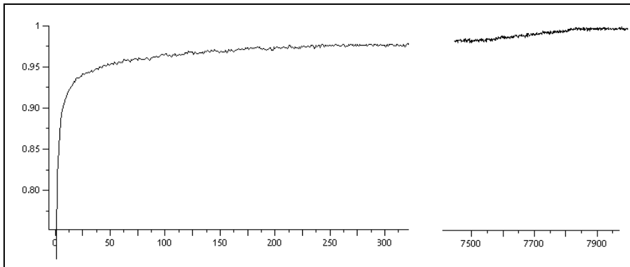
Figure 2: Convergence Diagnostics for Ising Gibbs Sampler
