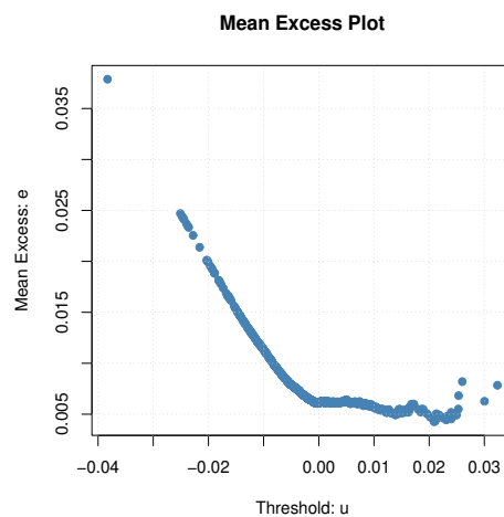
Figure 4. Mean excess plot of the S&P-500 dataset.
