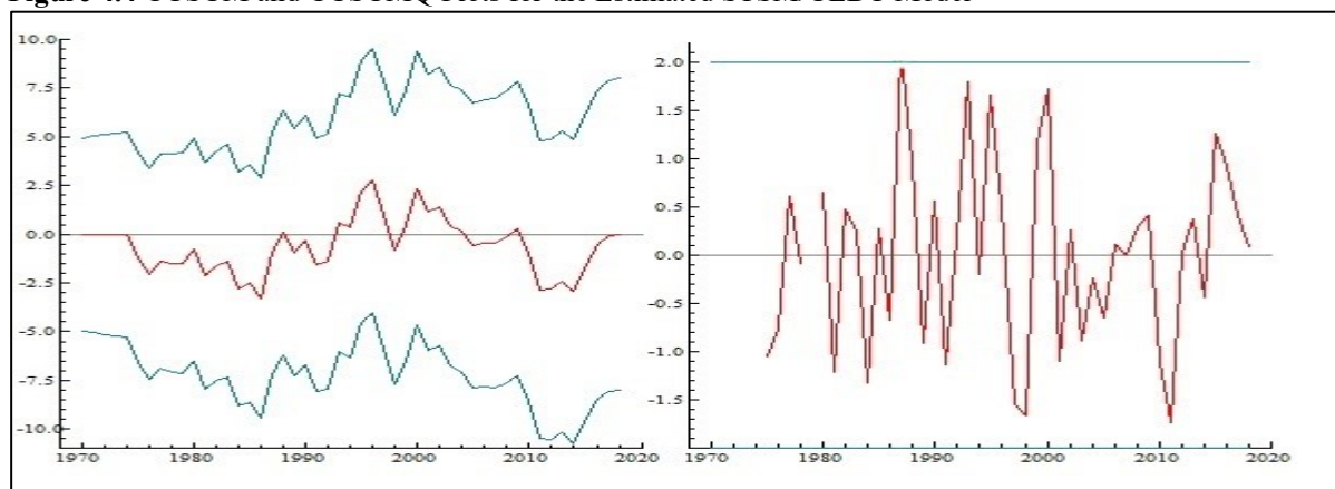
Figure 4.4 CUSUM and CUSUMQ Plots for the Estimated STSM/UEDT Model
