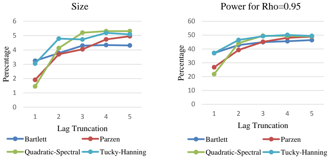
Figure 5.3 The Size and Power of MZ_a when Sample Size is 150 and \delta = 0.4 with DGP-I
