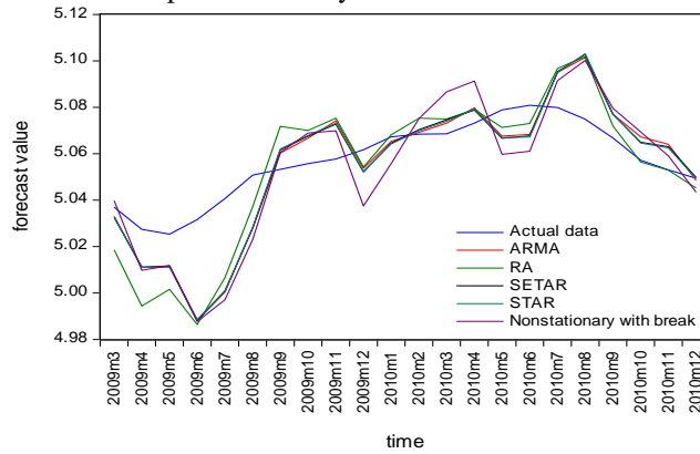
Figure 4.10 Four-step-ahead out-of-sample forecasts by the five models
