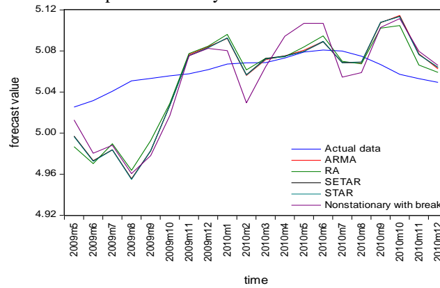
Figure 4.12 Six-step-ahead out-of-sample forecasts by the five models
