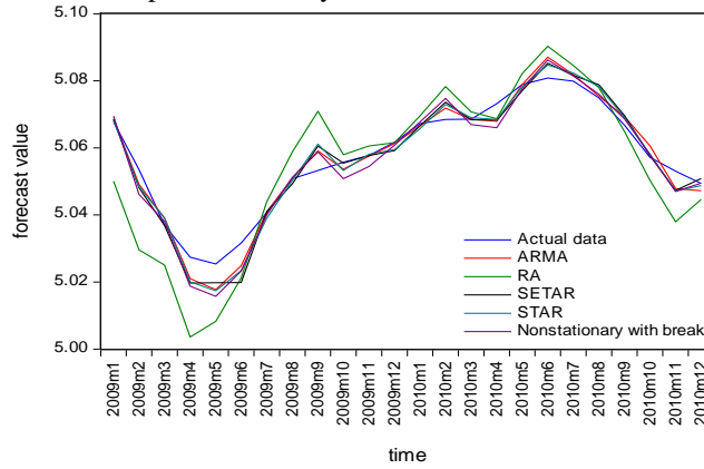
Figure 4.8 Two-step-ahead out-of-sample forecasts by the five models
