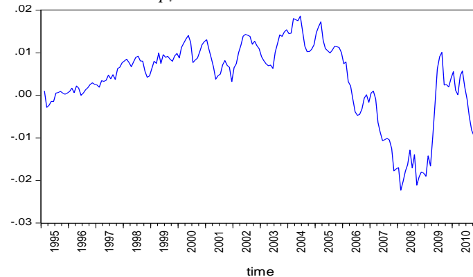
Figure 4.3 Plot of first differenced values of p_t
