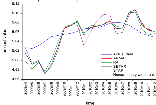
Figure 4.10 Four-step-ahead out-of-sample forecasts by the five models
