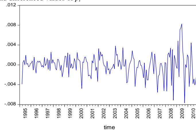
Figure 4.4 Plot of second differenced values of p_t
