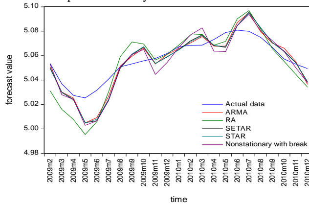
Figure 4.9 Three-step-ahead out-of-sample forecasts by the five models
