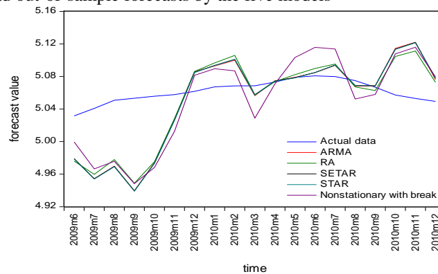
Figure 4.12 Six-step-ahead out-of-sample forecasts by the five models
