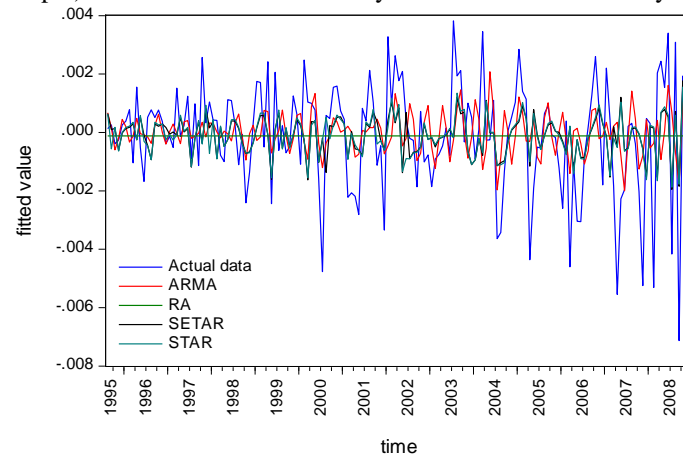
Figure 4.6a Fitted (in-sample) values of the four stationary models and the stationary data
