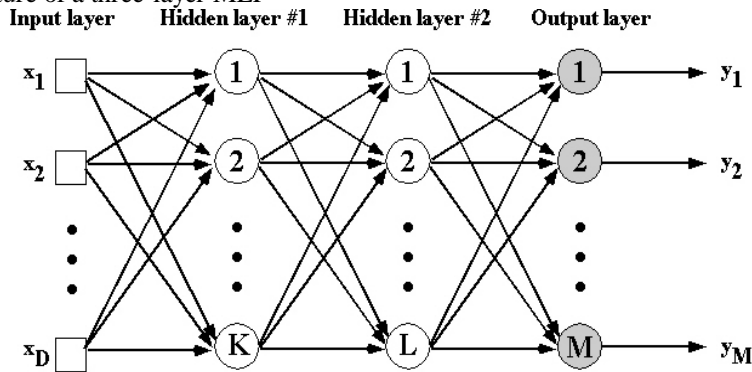
Figure 3.1 Architecture of a three-layer MLP
