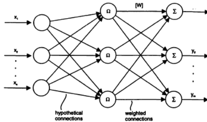
Figure 3.2 Architecture of a RBF Network
