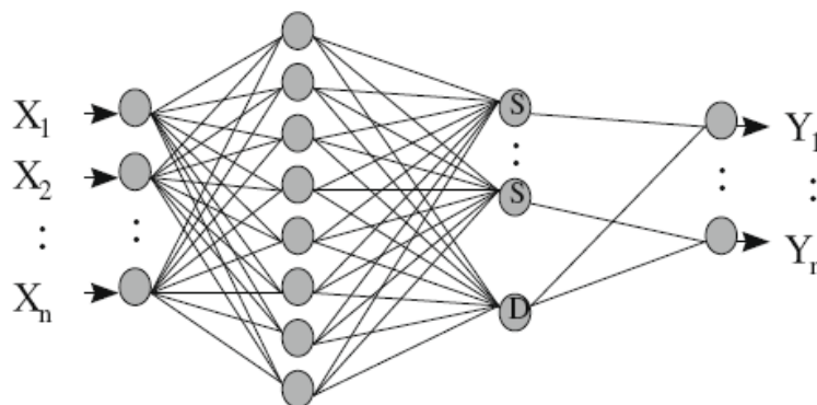
Figure 3.3 General structure of the GRNN
