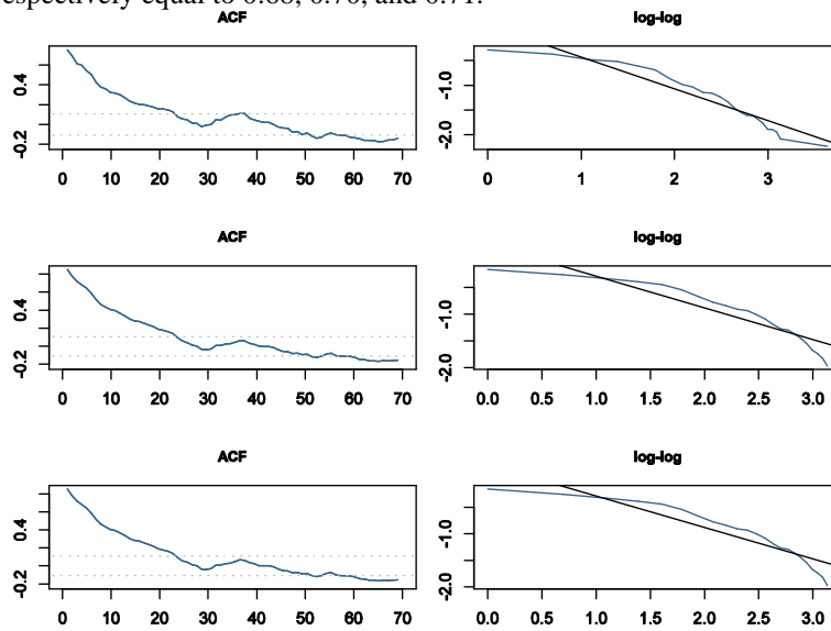
Figure 4.5 Autocorrelation function and long memory autocorrelation function plots of volatilities, computed based on returns on Euro/GBP data. For all functions of both kind of autocorrelation function and long memory autocorrelation function, the number of lags is arbitrarily equal to 70. The top row belongs to RS measure, the middle to RA, and the bottom to TSAV. Left plots are autocorrelation functions and right ones are long memory autocorrelation functions. Estimated Hurst exponent (self-similarity parameter) in long memory process for RS, RA, and TSAV are respectively equal to 0.68, 0.70, and 0.71.
