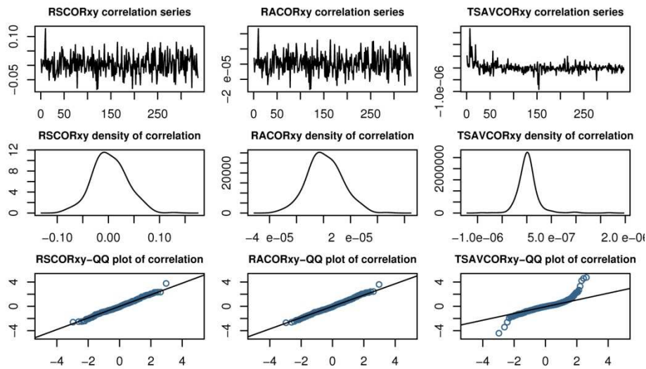
Figure 4.3 Distributional properties of realized correlations between Euro/USD and Euro/GBP are graphically embodied. Evidently realized correlations, based on first row plots, fluctuate over the time. The correlations oscillate almost around zero mean. The RS and RA based correlations possess a near symmetric density approximately with zero mean, while density of the other is positively skewed. These findings are more informatively supplemented by QQ-normal plots. Both RS and RA based correlations seem to shape a normal distribution.
