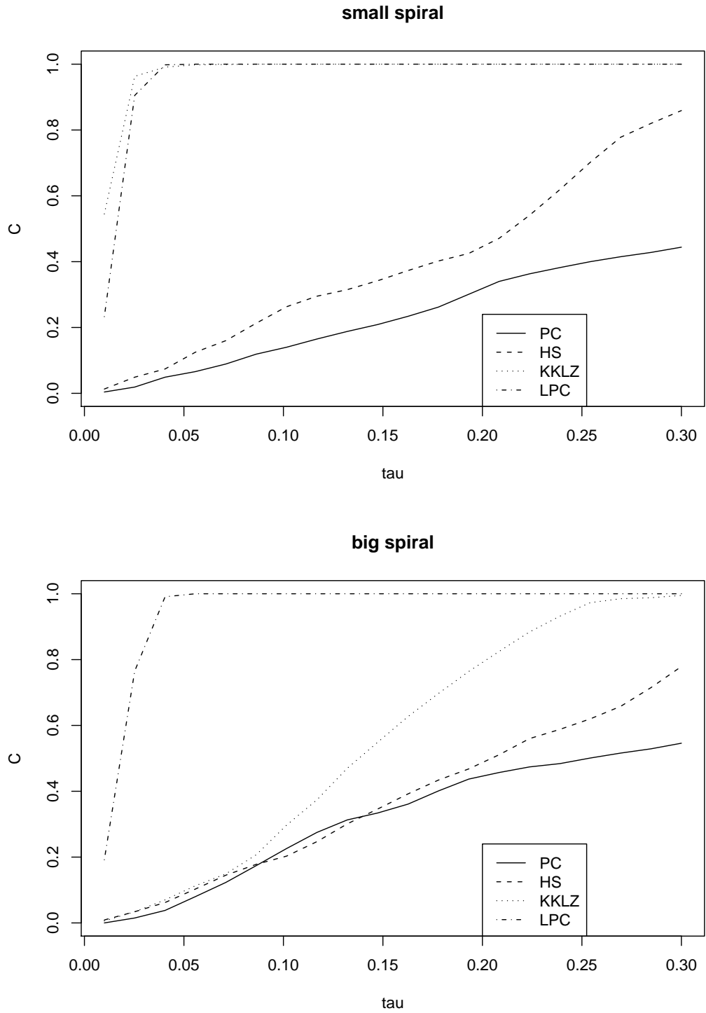
Figure 8: Coverage for small (top) and big (bottom) spiral data.
