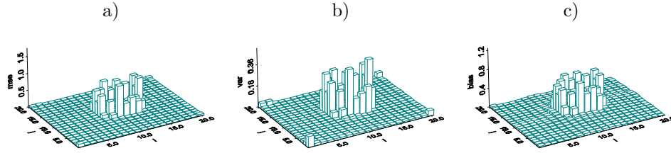
Fig. 10. compound Laplace with c=100 , d=20 a) MSE, b) variance, c) absolute bias
