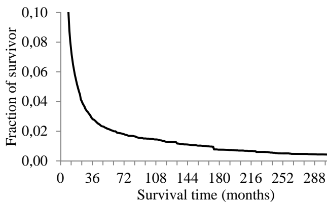
Figure 1: Kaplan-Meier survival functions
