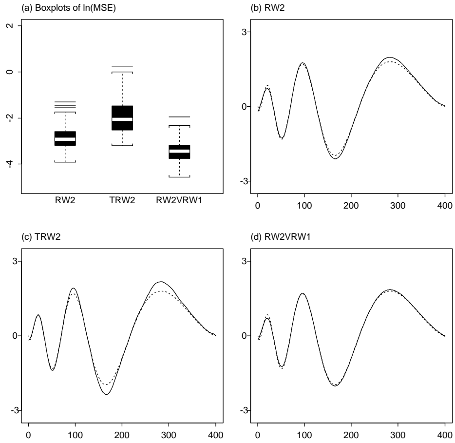
Figure 7: Simulation results for regression function with differing curvature and three observations on each design point. (a) Boxplots of \ln(\text{MSE}) . (b)-(d) Averaged posterior mean estimates (—) together with true function ( \cdots ).
