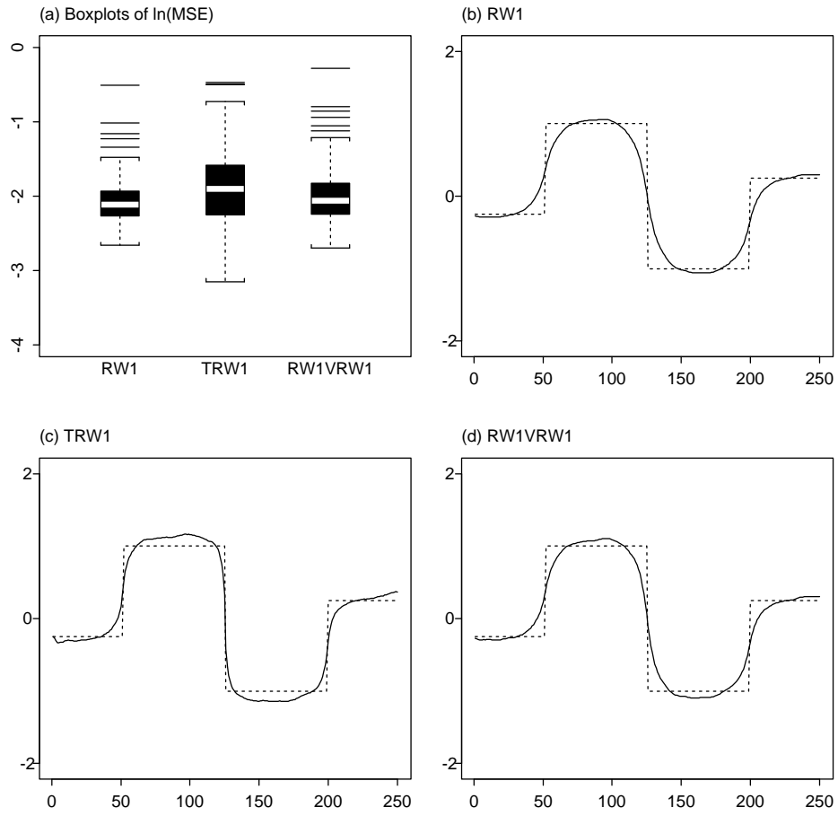
Figure 2: Simulation results for regression function with discontinuities and one observation on each design point. (a) Boxplots of \ln(\text{MSE}) . (b)-(d) Averaged posterior mean estimates (—) together with true function ( \cdots ).
