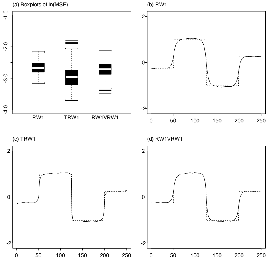
Figure 3: Simulation results for regression function with discontinuities and three observations on each design point. (a) Boxplots of \ln(\text{MSE}) . (b)-(d) Averaged posterior mean estimates (—) together with true function ( \cdots ).
