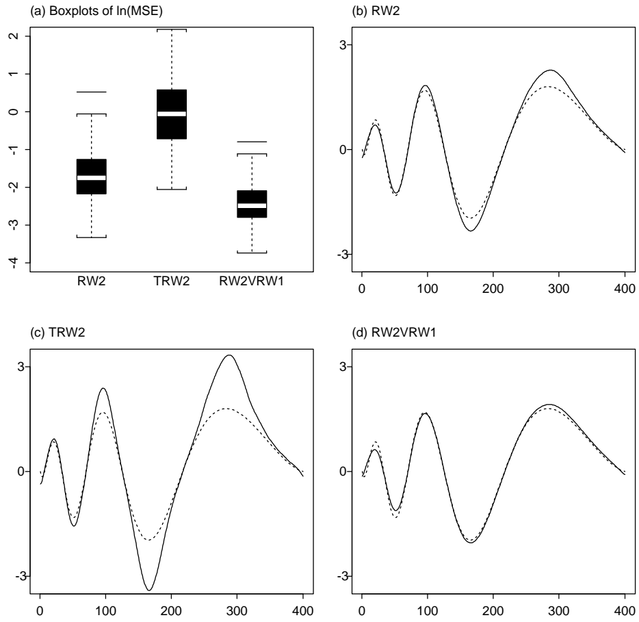
Figure 6: Simulation results for regression function with differing curvature and one observation on each design point. (a) Boxplots of \ln(\text{MSE}) . (b)-(d) Averaged posterior mean estimates (—) together with true function ( \cdots ).
