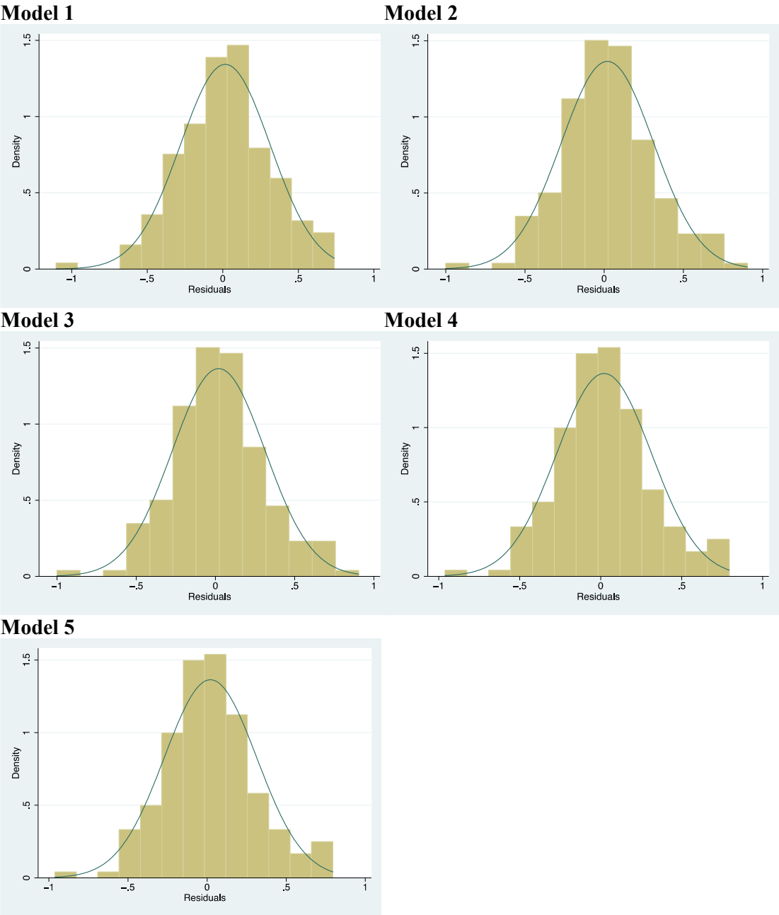
Figure 13. Residual-based Normality Plots for MGB10Y, CETES3M, CCPI, and IP
