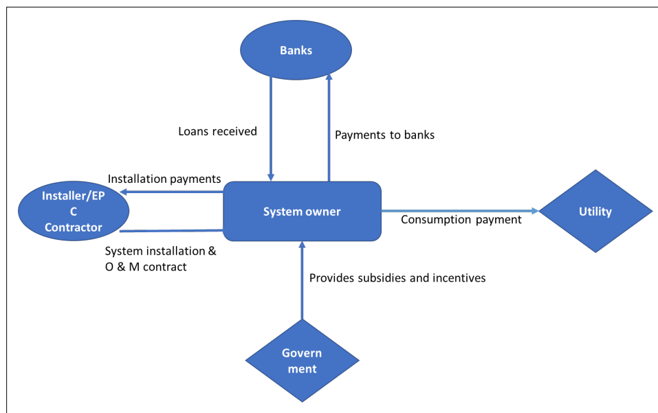
Figure 4: CAPEX Model
