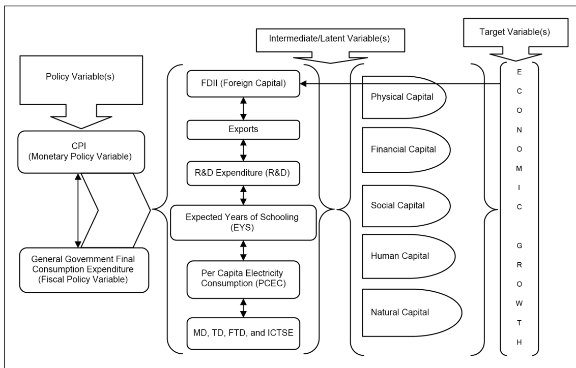
Figure 2: Theoretical Relationship
