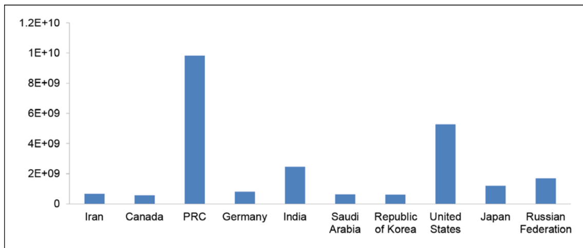
Figure 4: CO 2 Emissions
