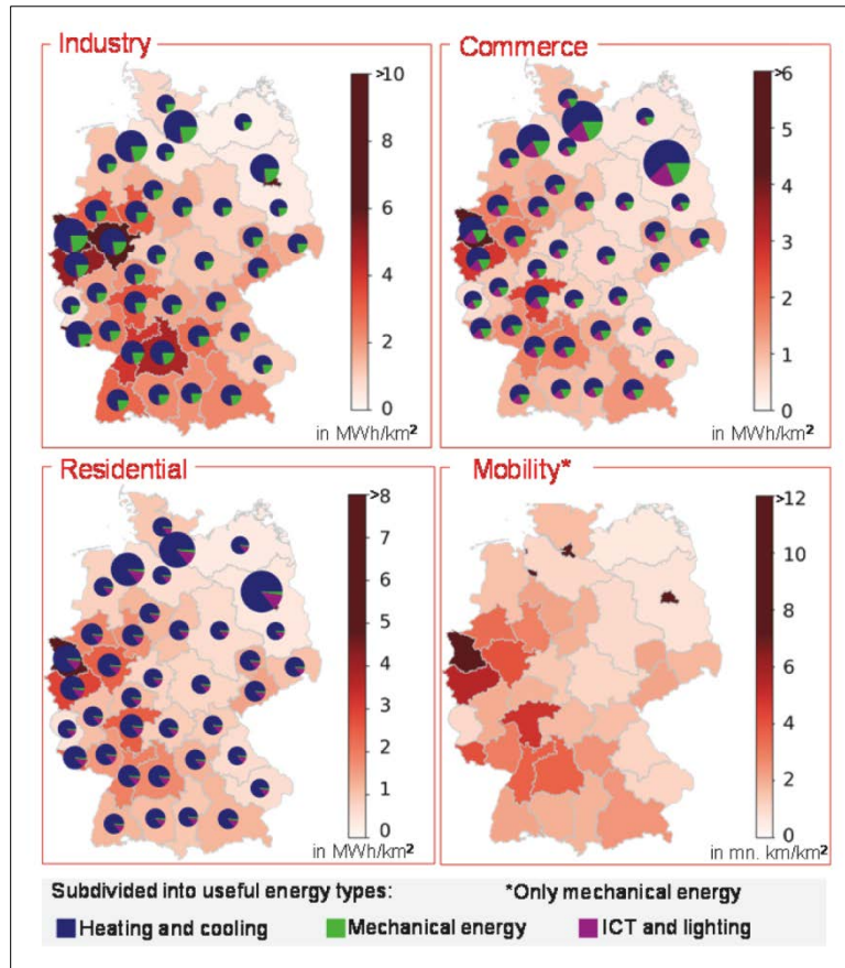
Figure 12: Regional Distribution of Useful Energy Demand for the Different Sectors in Germany for the 95% GHG Emission Reduction Scenario Divided into Useful Energy Types Except for Mobility (Only Mechanical Energy)
