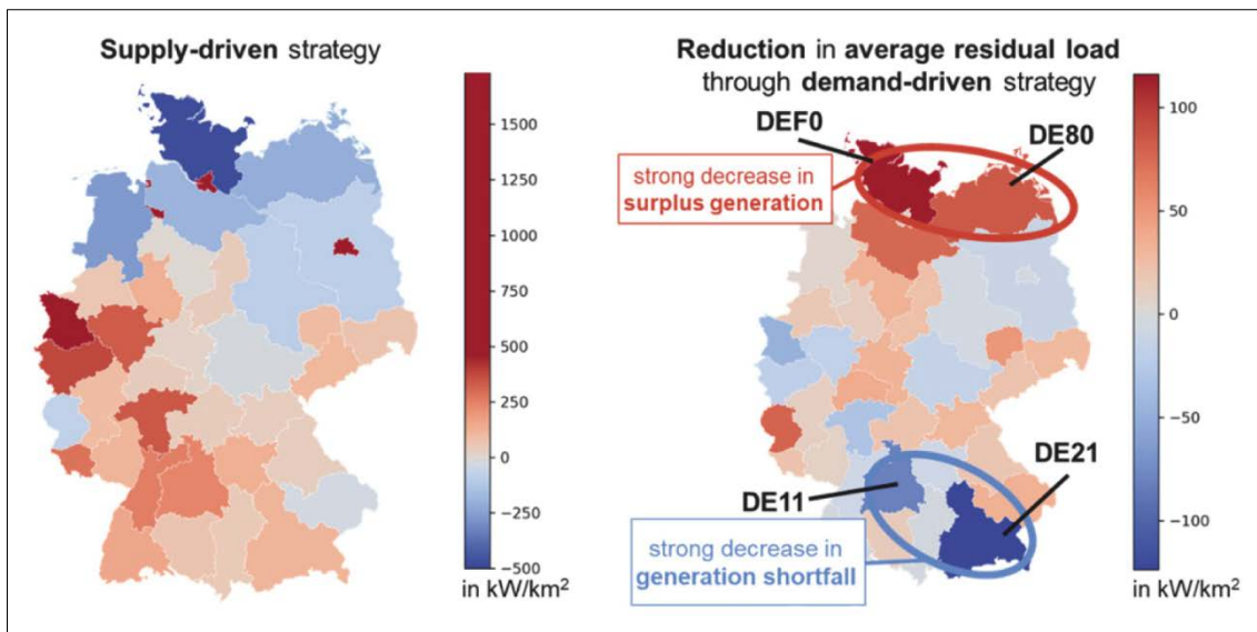
Figure 15: Average Residual Load for 95% GHG Emission Reduction Scenario for the Supply-Driven and Demand-Driven Strategy
