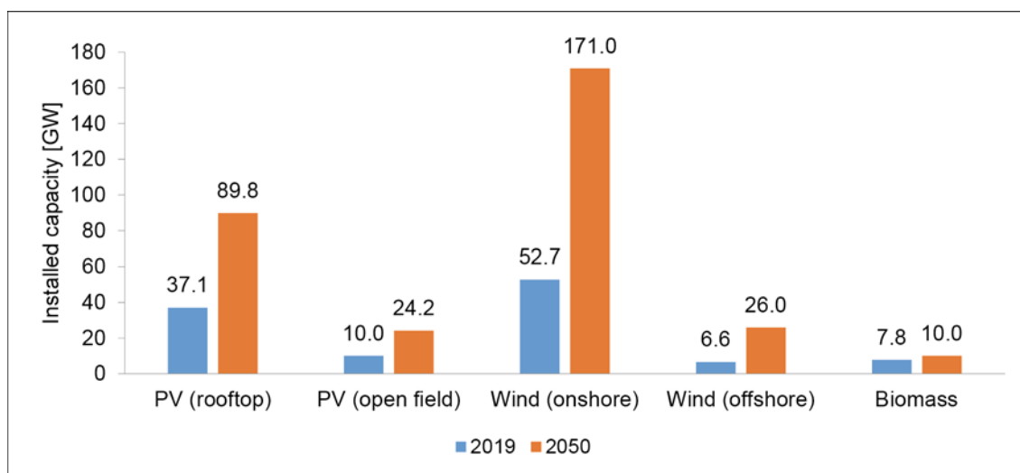
Figure 10: Renewable Power Generation Capacities for the Status Quo and the Scenario Under Investigation
