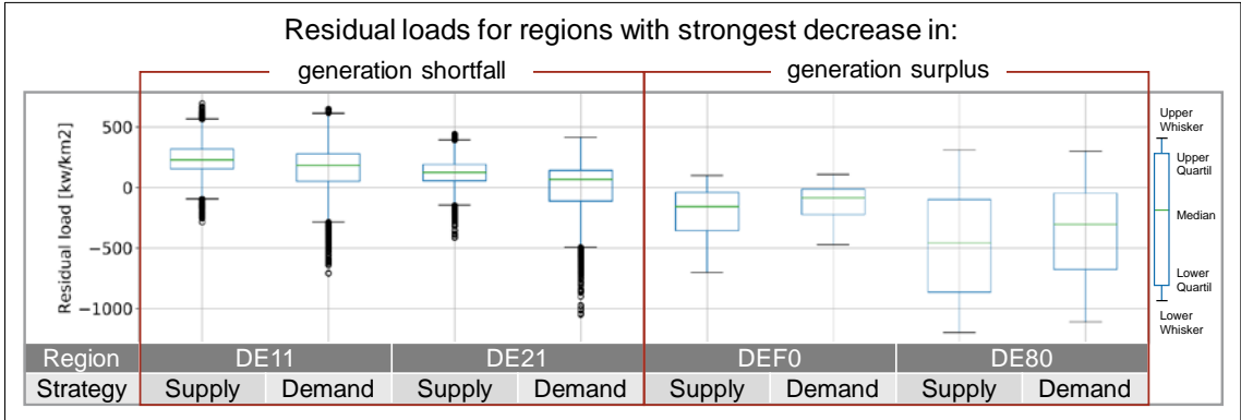
Figure 16: Boxplots for the Resulting Residual Load in Four Exemplary NUTS2 Regions for Supply-Driven and Demand-Driven Strategy (Here Shortened to Supply and Demand)
