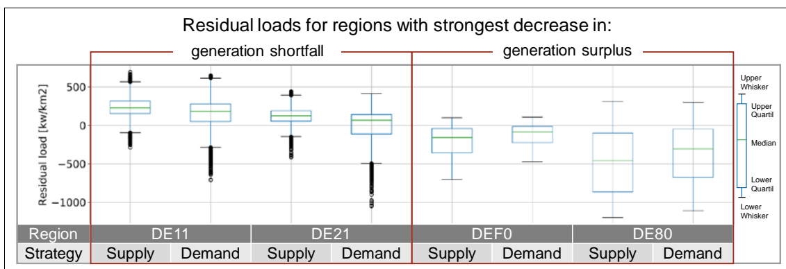
Figure 16: Boxplots for the Resulting Residual Load in Four Exemplary NUTS2 Regions for Supply-Driven and Demand-Driven Strategy (Here Shortened to Supply and Demand)
