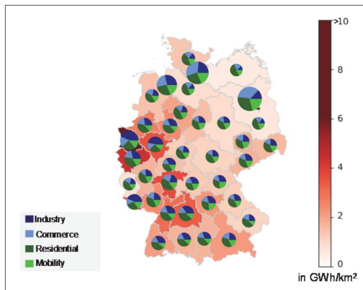
Figure 13: Electricity Demand per Sector for the 95% GHG Emission Reduction Scenario
