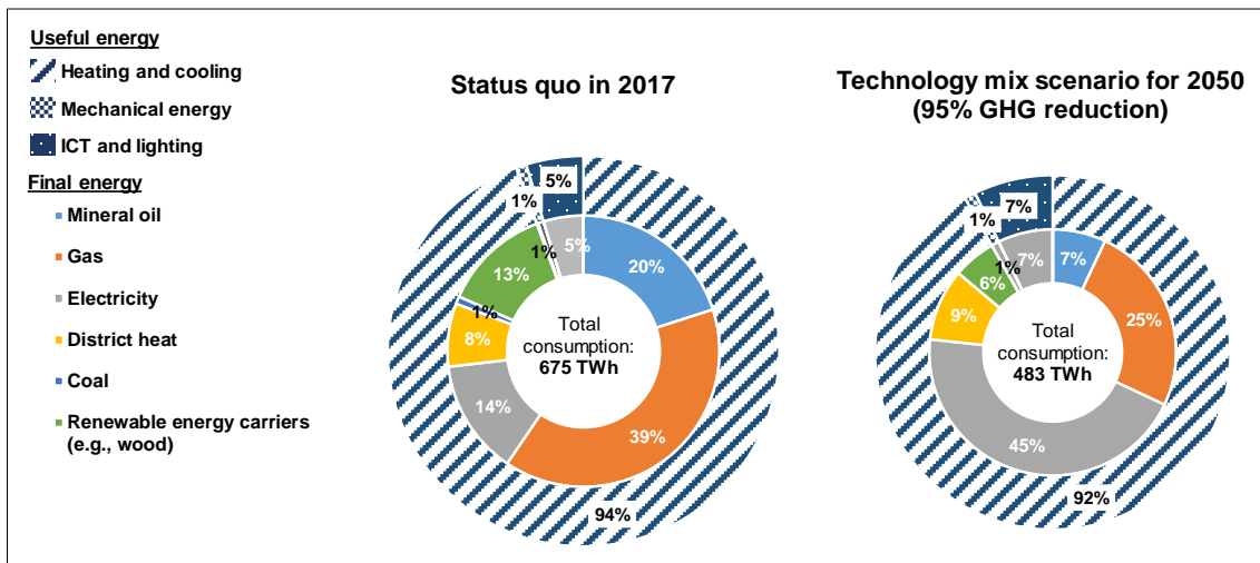
Figure 8: Final Energy Demand in the Residential Sector. Own Calculation and Illustration
