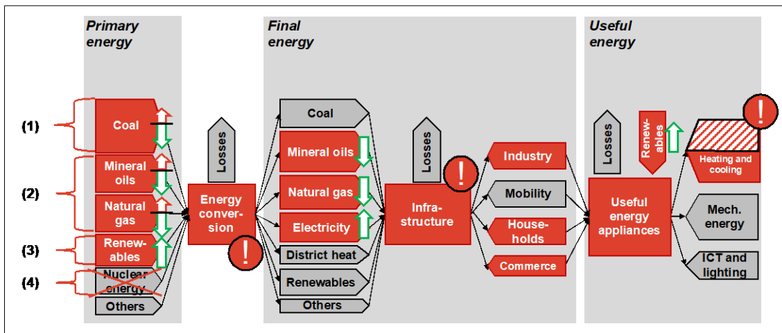
Figure 2: Integration of Heat Pumps into the Energy System
