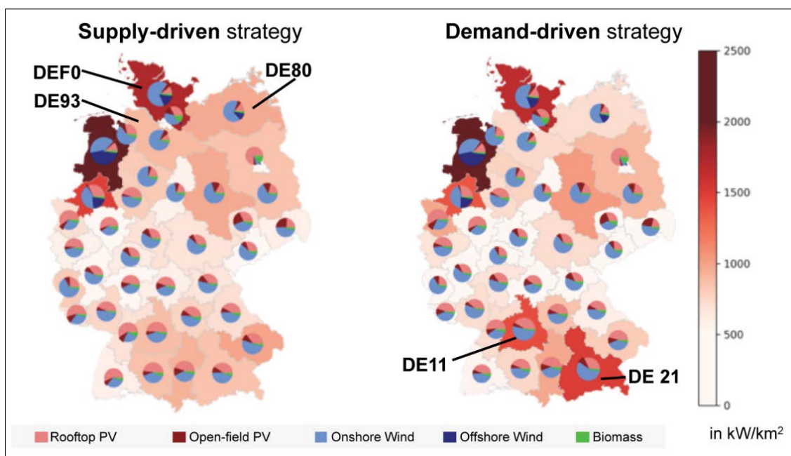
Figure 14: Renewable Electricity Generation Capacities According to the 95% GHG Emission Reduction Scenario for the Supply-Driven Strategy and the Demand-Driven Strategy
