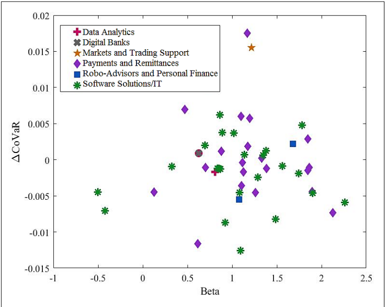
Figure B.5: European Fintech: \Delta\text{CoVaR} and Beta
