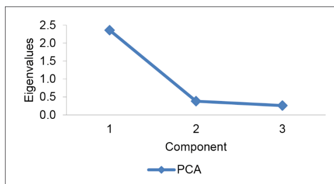
Figure B1: Scree Plot Graphs of the Amount of Variation Explained by Each Component
