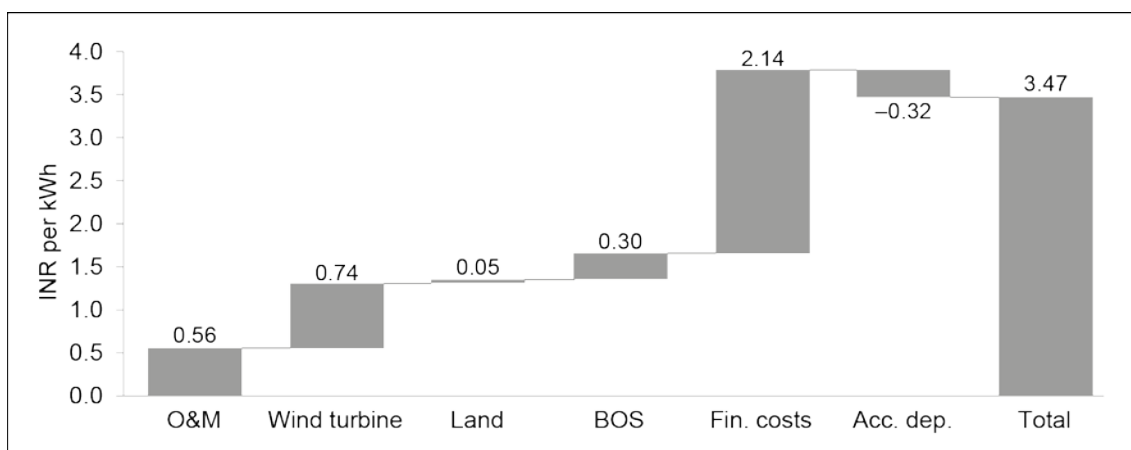
Figure 2: Financing Costs Constitute the Largest Component of Indian Wind Energy Tariffs
