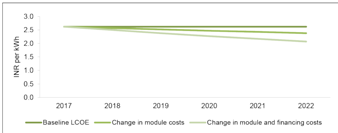
Figure 4: Financing Costs Increasingly Important in Order to Lower LCOE Going Forward
