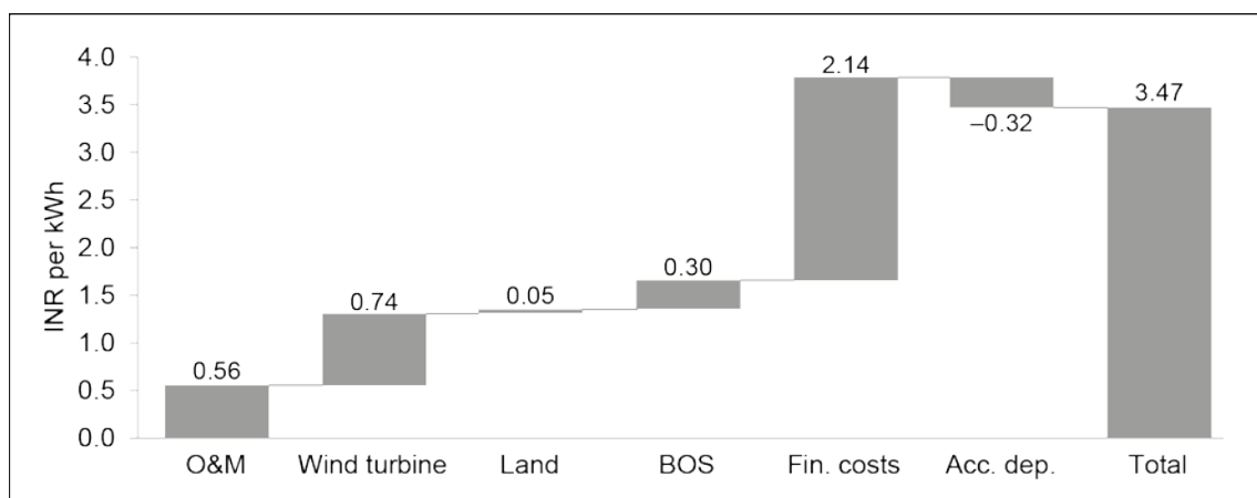
Figure 2: Financing Costs Constitute the Largest Component of Indian Wind Energy Tariffs
