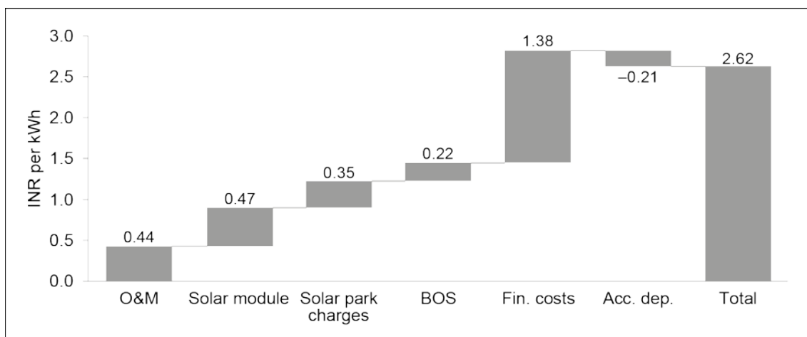
Figure 3: Financing Costs Constitute the Largest Component of Indian Solar Energy Tariffs
