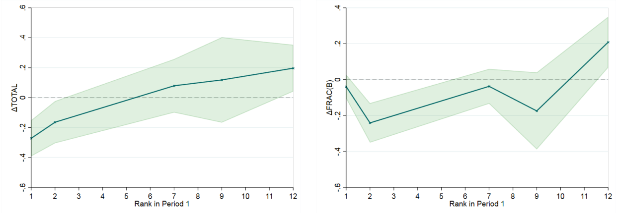
Figure B4: Percentage changes in the absolute number of solved items in total ( \Delta_{\text{TOTAL}} ; left) and in the fraction of solved items in Domain B ( \Delta_{\text{FRAC(B)}} ; right) from period 1 to period 2 as a function of rank in period 1. Shaded areas represent 95% confidence intervals.
