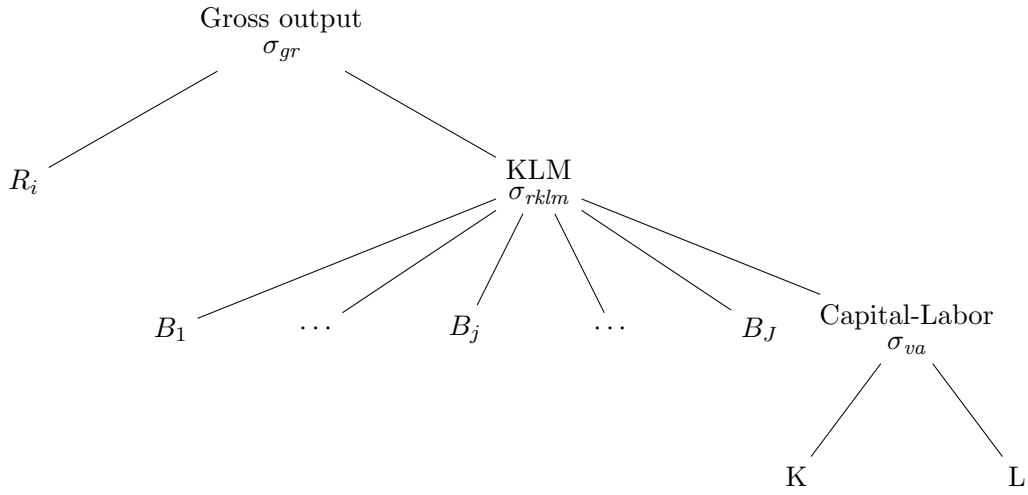
Figure A3. Production structure of energy resource sectors f \in F \subset P\{\text{COL,CRU,GAS}\} .
