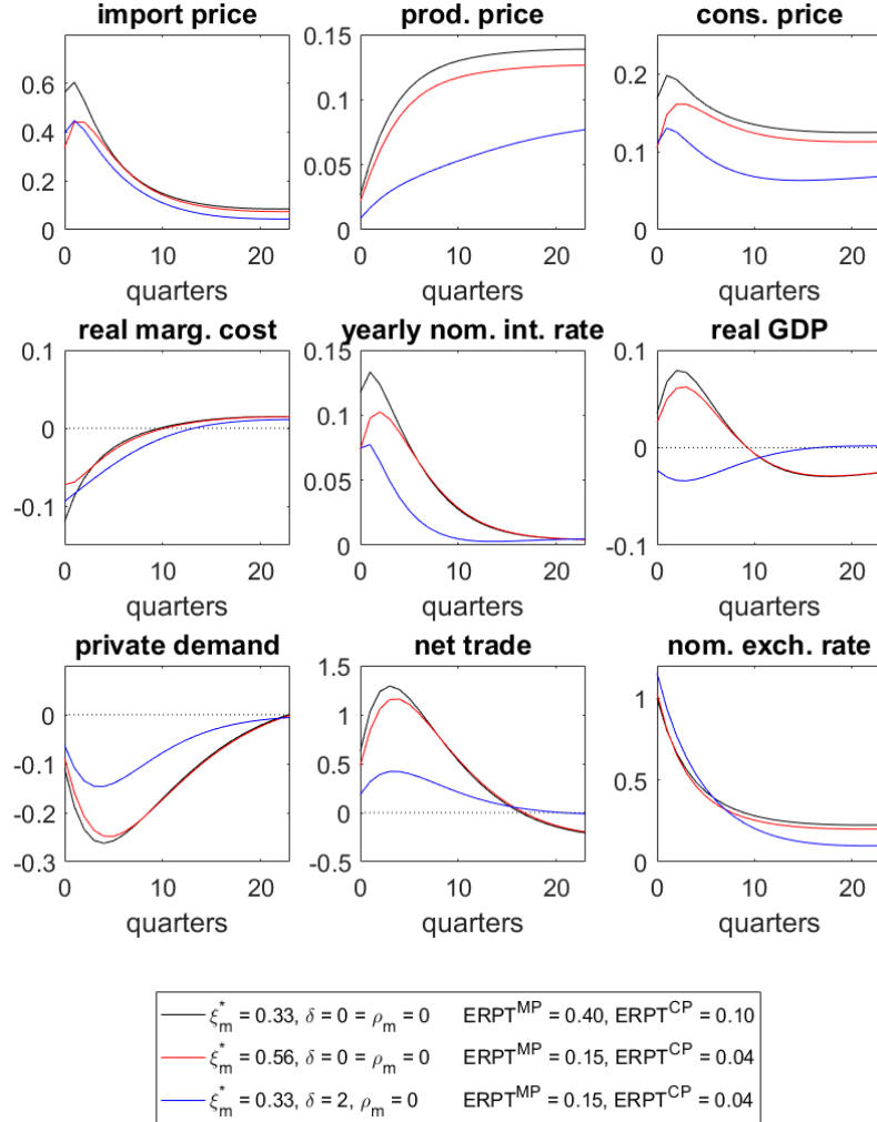
Figure 6: EA impulse responses to a 1% euro depreciation import price nominal stickiness vs distribution
