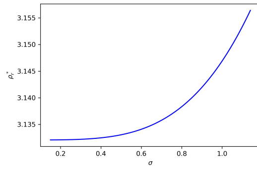
(B) Discounted MFG with r = 0.5 : \rho_r^* vs. \sigma
