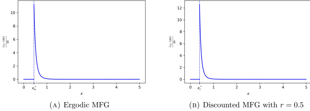
FIGURE 1. Density functions of the stationary distributions in equilibrium
