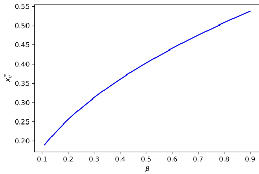
(A) Ergodic MFG: x_e^* vs. \beta
