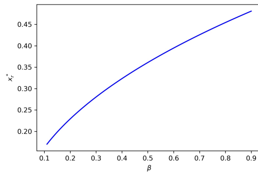
(B) Discounted MFG with r = 0.5 : x_r^* vs. \beta
