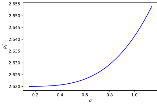
(A) Ergodic MFG: \rho_e^* vs. \sigma
