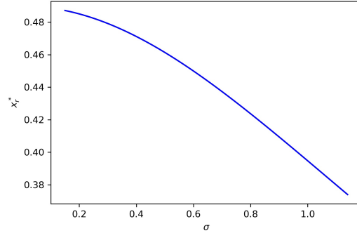
(B) Discounted MFG with r = 0.5 : x_r^* vs. \sigma
