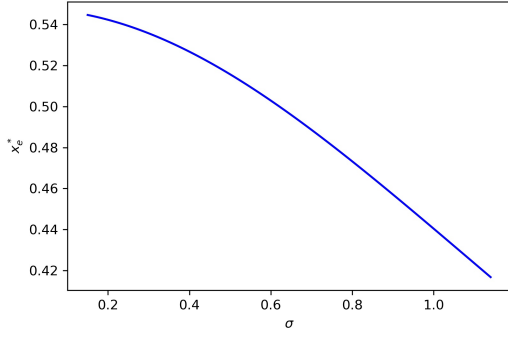
(A) Ergodic MFG: x_e^* vs. \sigma
