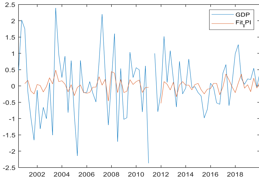
Figure 6: U-Midas (In-Sample Fit) IPI
