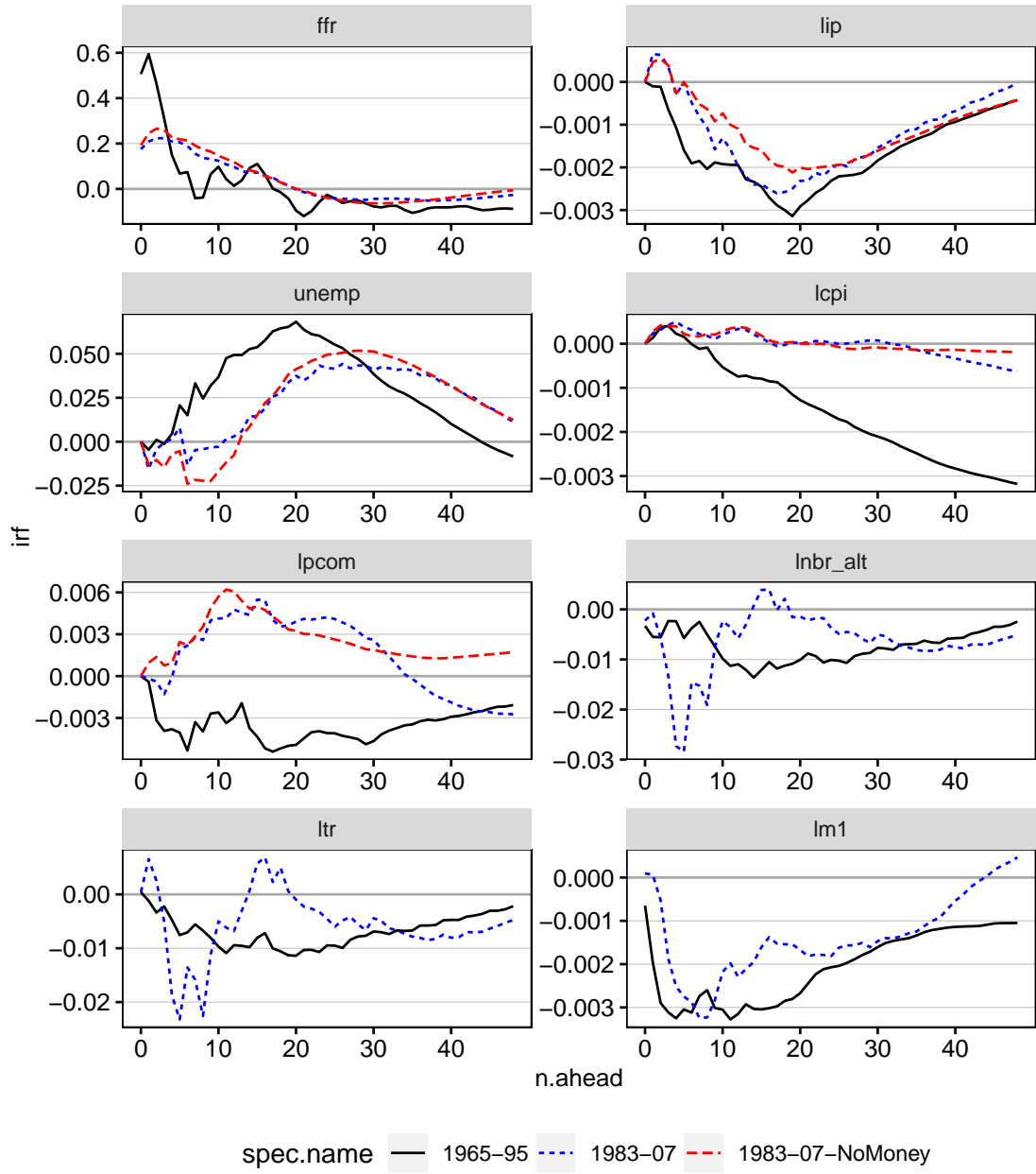
Figure 2: Update
