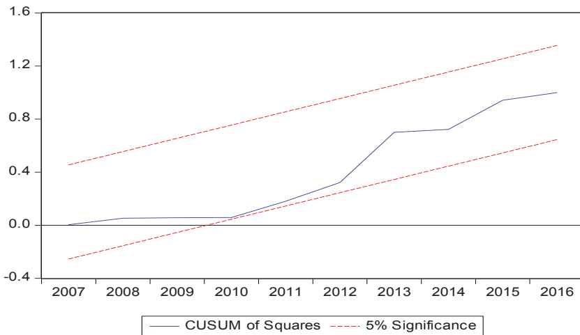
Figure 8. Cumulative sum of squares (CUSUMQ).
