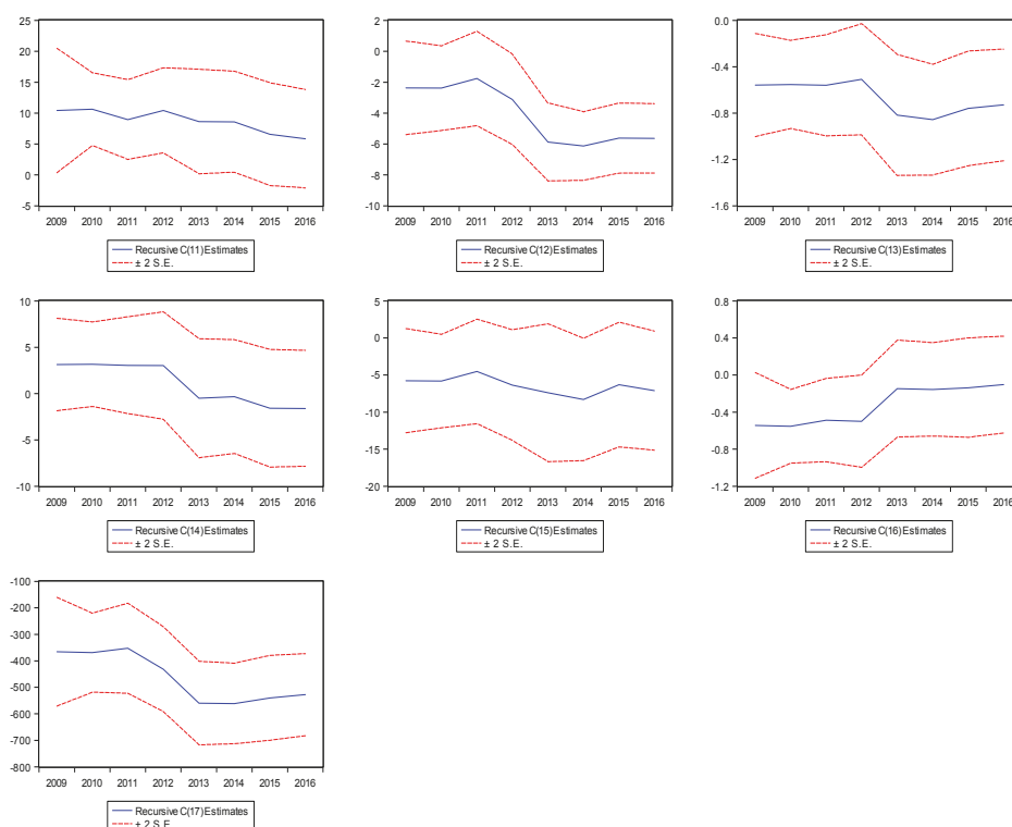
Figure 9. Recursive least squares graphs for the long-run model.
