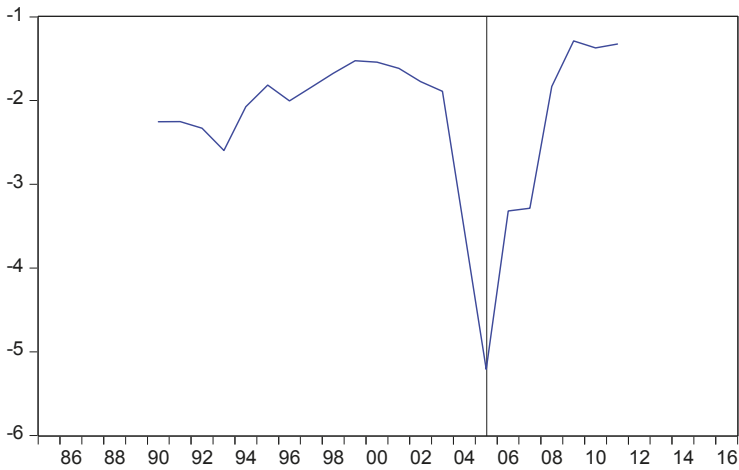
Figure 6. Zivot-Andrew breakpoints test results.
