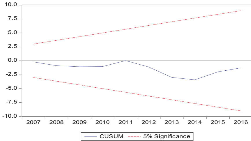
Figure 7. Cumulative sum (CUSUM).
