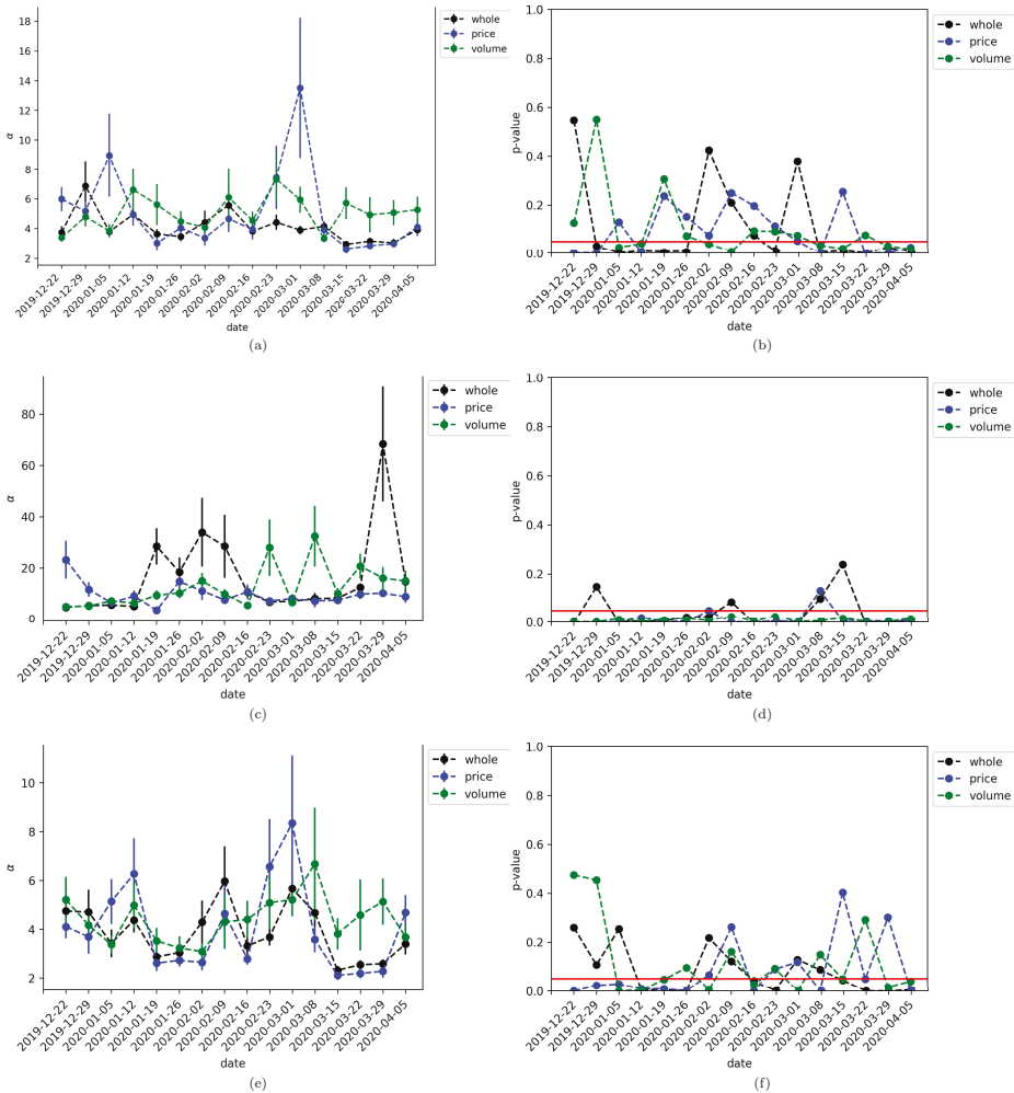
Figure 3. The Behavior of the mTE network structure through time. (a,b) show the dynamic of the estimated power \alpha and corresponding p -value for the degree distribution. (c,d) show the dynamic of the estimated power \alpha and corresponding p -value for the in-degree distribution. (e,f) show the dynamic of the estimated power \alpha and corresponding p -value for the out-degree distribution. In all cases, the black line represents the results for the whole network, the blue line for the price-returns subgraph, and the green line for the volume-returns subgraph. The red straight line is the significance threshold of 0.05 and the vertical lines centered at each point represents the standard deviations.
