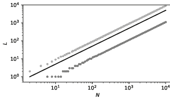
Figure 8. Dependence of L(= N_L^{CXmax}) vs. N . There are two solutions of Equation (30): one marked with blue circles and the other with orange ones. Above N \approx 10^2 , both dependencies are linear, which is particularly clearly confirmed in Figure 9. That is, in a log-log scale, their slopes equal 1. However, in linear scale, the directional coefficients of these straight lines equal 0.11 and 0.89, respectively. This is clearly shown in Figure 9. Only the solution with orange circles is realistic, because the chance that 89% of particles will pass in a finite time to the second part of the container (as indicated by the solution marked with blue circles) is negligibly small. The black solid tangent straight line indicates a reference case N_L^{CXmax} = N/2 .
