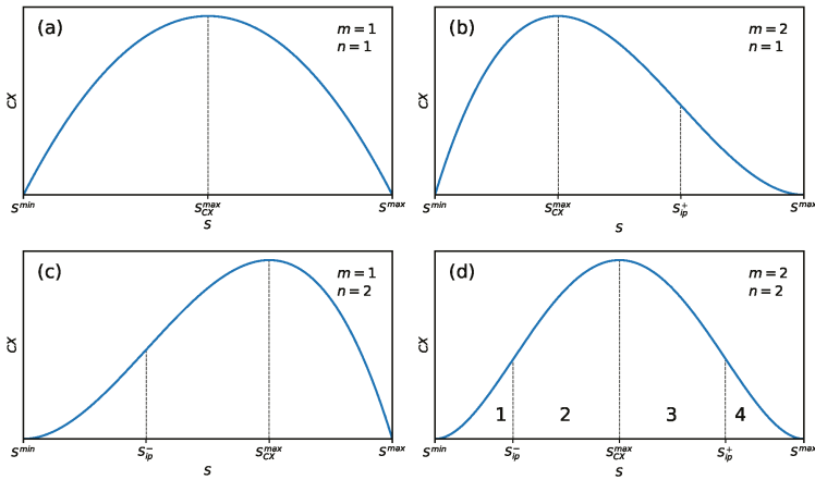
Figure 1. Plots of the partial measure of complexity CX(S; m, n) vs. S given by Equation (1) for four characteristic cases: (a) Case n = m = 1 where no inflection points, S_{ip}^{\mp} are present. (b) Case m = 2 and n = 1 where a single inflection point S_{ip}^+ is present. (c) Case m = 1 and n = 2 where a single inflection point S_{ip}^- is present. (d) Case m = 2 and n = 2 where both inflection points are present. The shape of the curve, containing two inflection points, is typical for partial measures of complexity, characterized by exponents m, n \geq 2 . Numbers 1–4 mark individual phases differing in the degree of order.
