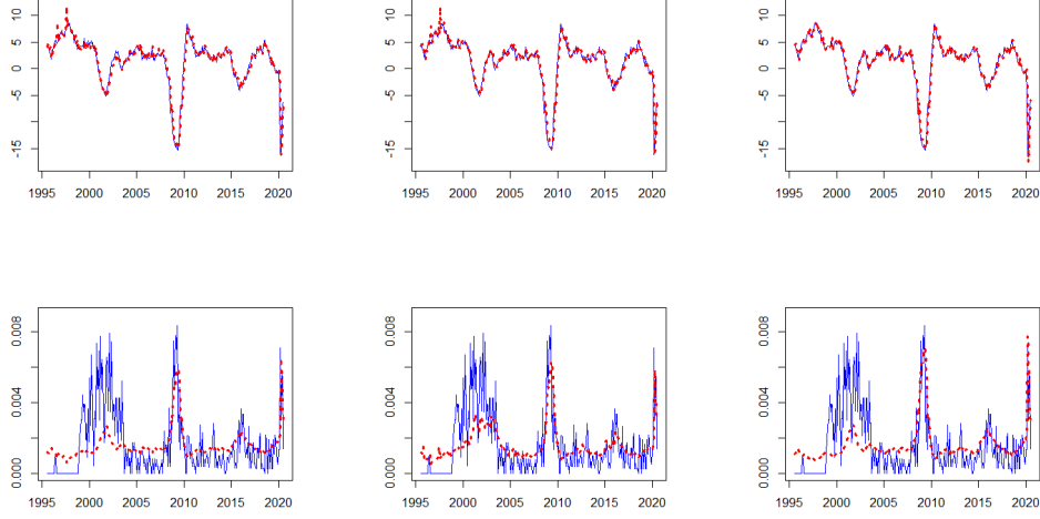
Figure 4: Macro fit (top row) and NP-D fit for model 3, 4 and 5
