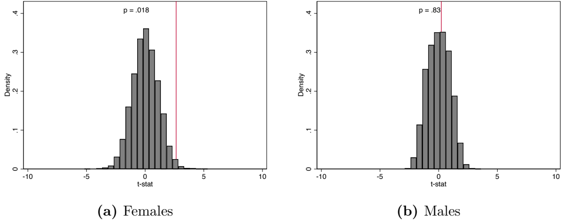
Figure 5. Pseudo-treatment Effects
