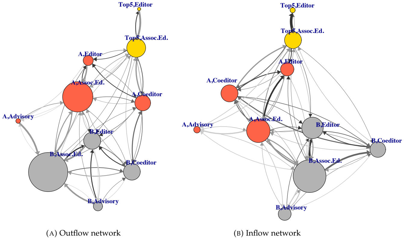
FIGURE 6. Editorial moves
