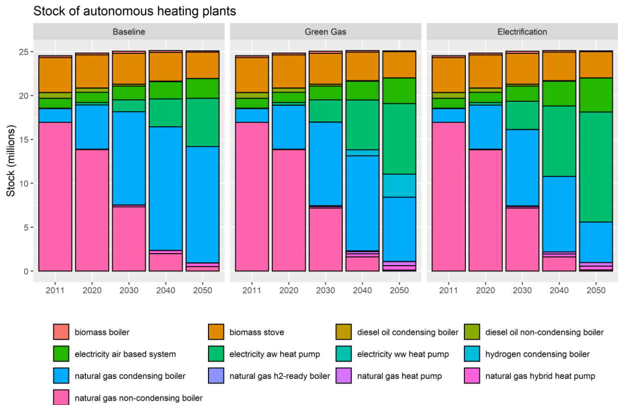
Figure 3 – Total stock of autonomous heating plants, by technology and by scenario.
