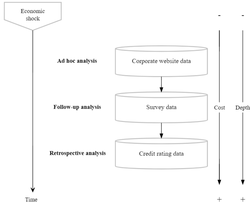
Figure 1: Framework visualization
