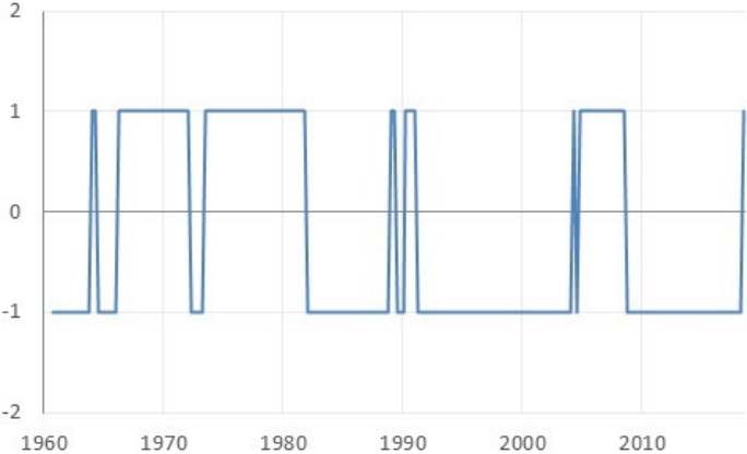
Figure 5: Evolution of adjusted PCE inflation minus sample period average
