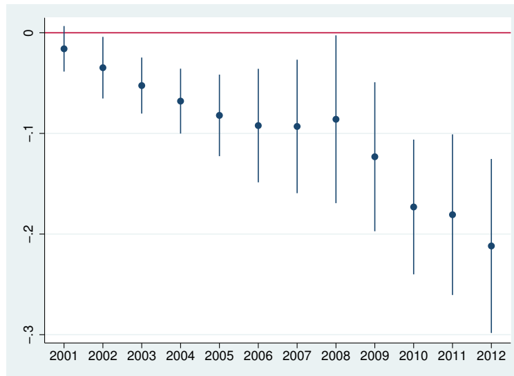
Figure 4: Year Dummies
