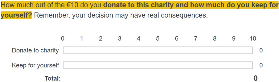
Figure 2: Sliders used to elicit donation in sequential dictator games
