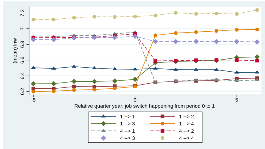
Figure A3: Event study 52 of Card et al. (2013)
