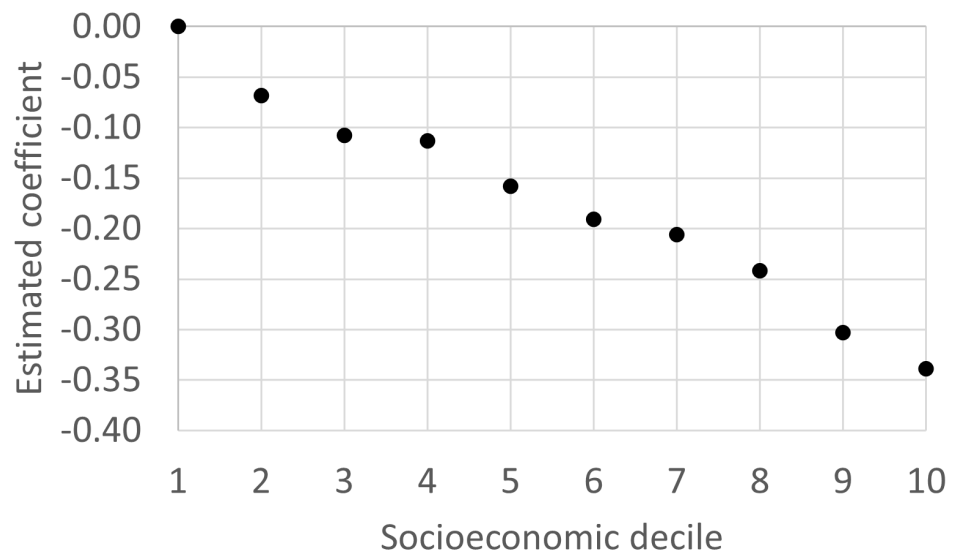
Figure 4: Estimated Coefficients for Nonlinear Model (Bogotá)
