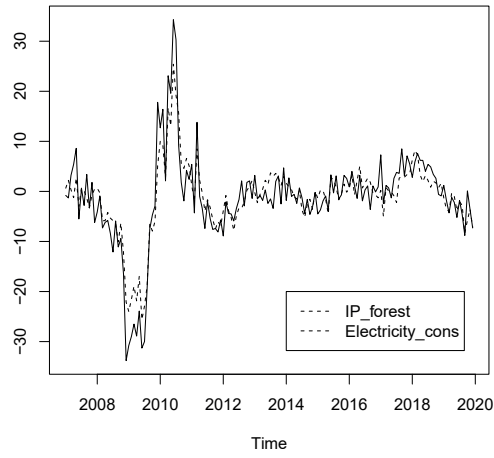
(b) Corr=0.94
