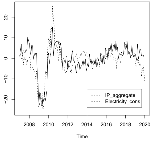
(a) Corr=0.69
