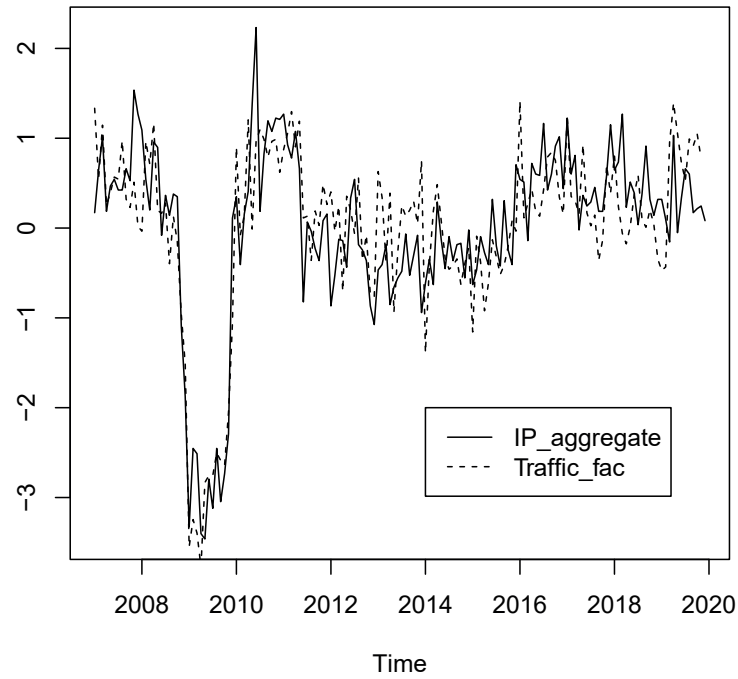
Figure 3: Year-on-year growth rate of the volume index of industrial production, working-day adjusted, and the first factor extracted from data on truck traffic volumes. The series are standardized and they cover the period from 2007 to December 2019.
