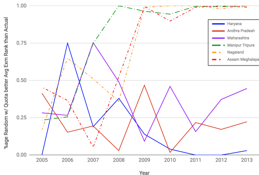
Figure 5. Comparing Average Exam Rank for Selected Cadres with Random Allocations.
