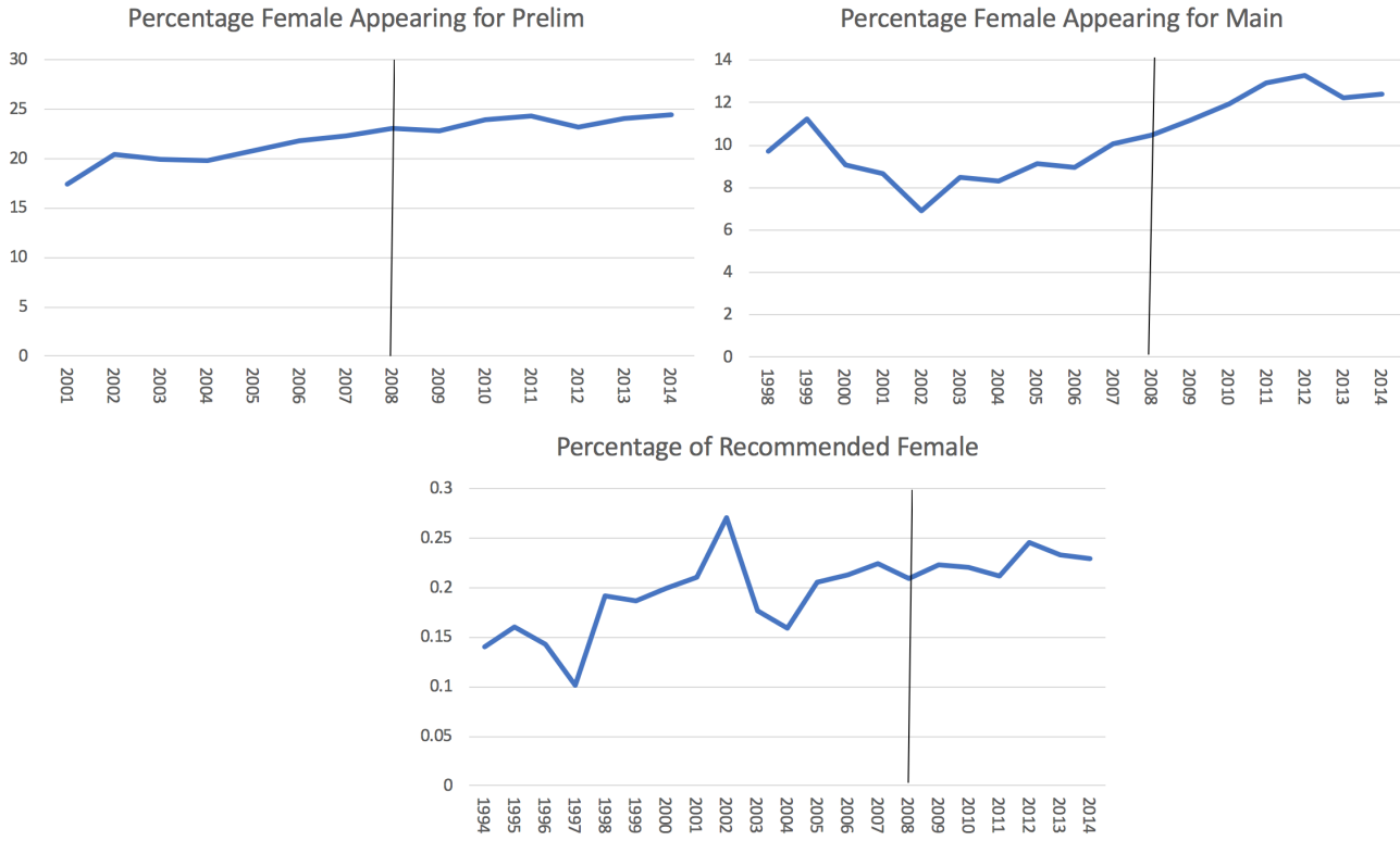
Figure 54. Gender balance in CSE and IAS.
