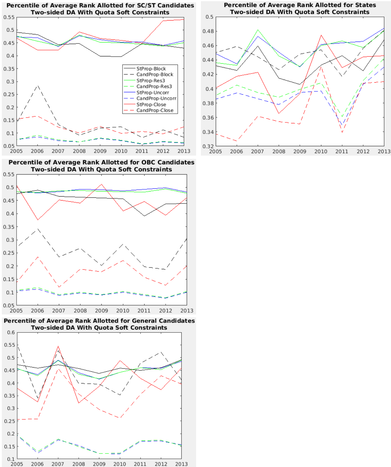
Figure 40. Percentile of average preference rank allotted under Two-sided DA with quota soft constraints.
