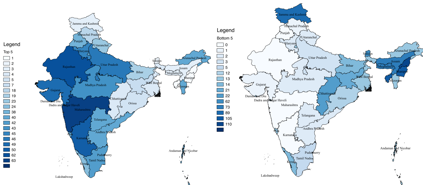
Figure 50. Top and bottom 5 cadre preferences for IPS 2008 batch.
