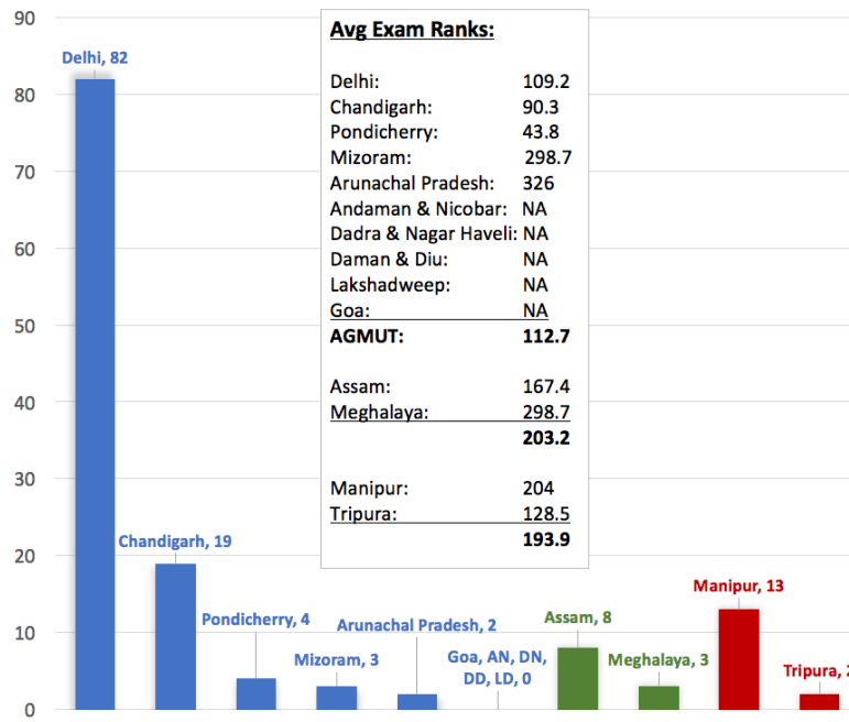
Figure 33. Origin and Average Exam Rank of Exam Toppers from Joint Cadres.
