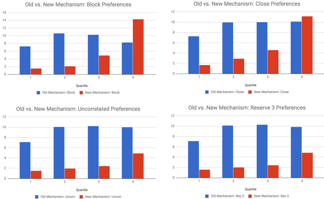
Figure 19. Average preference rank for each exam quartile with Old vs. New Mechanism under various preference structures.
