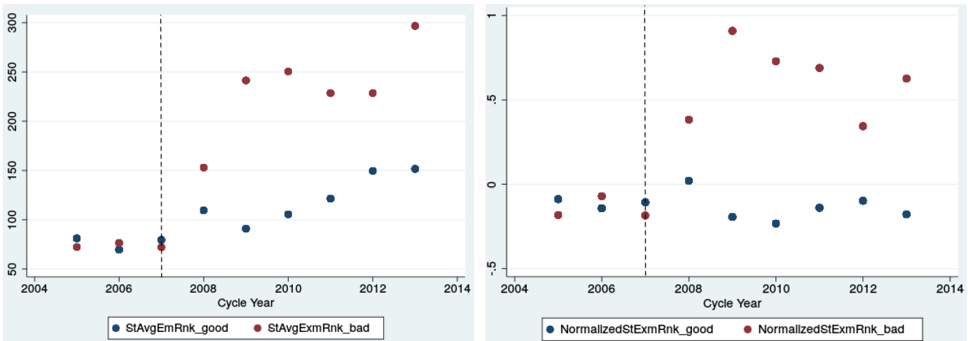
Figure 9. Effect of New Mechanism on Average Exam Rank across Good and Bad Cadres.
