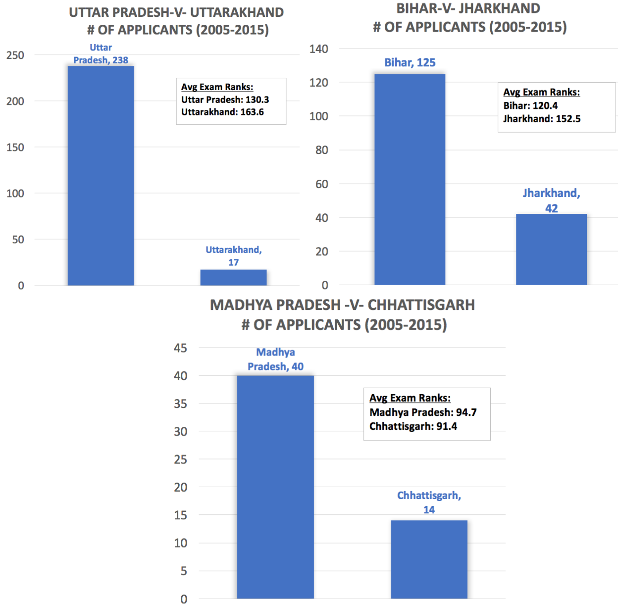
Figure 32. Exam toppers from States which split in 2000.
