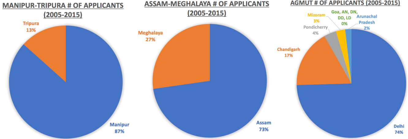
Figure 31. Origin of Exam Toppers Amongst Joint Cadres.
