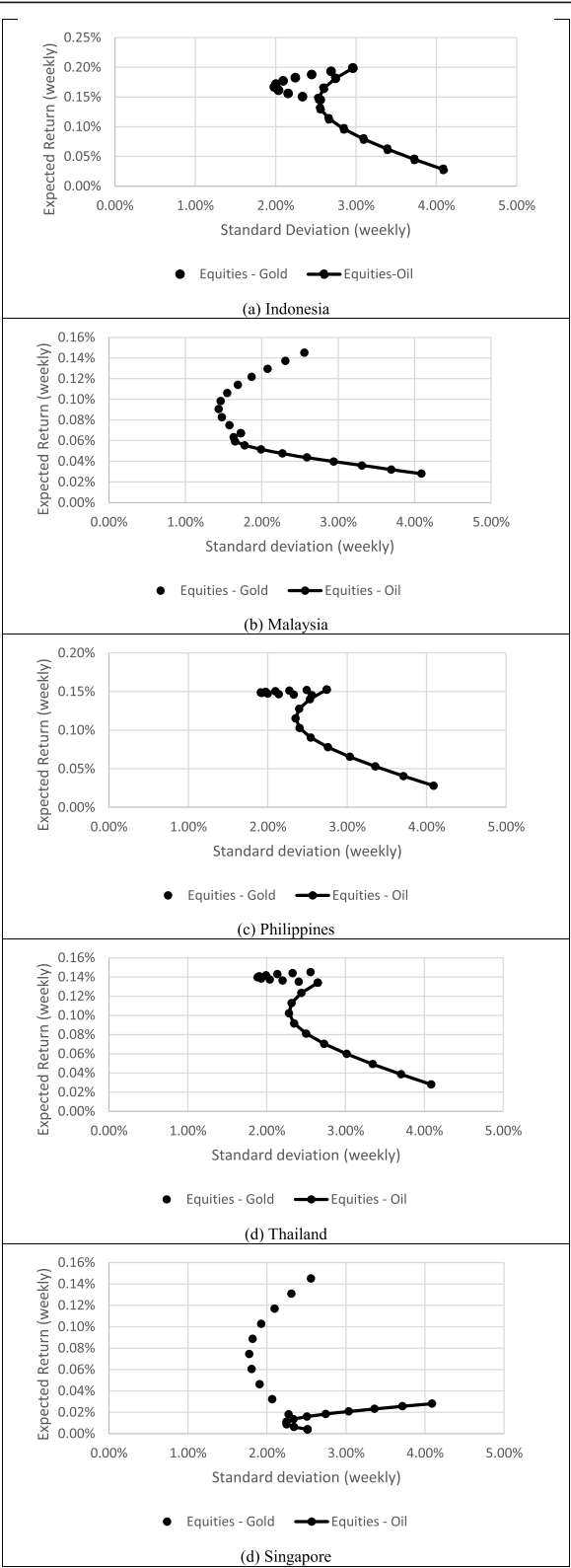
Fig. 5 Minimum Variance Portfolio
