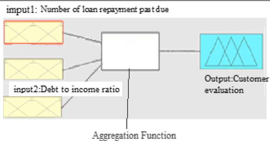
Fig. 18 Aggregation function. The aggregation function was defined to map the inputs such as input1 (number of loan repayment past due) and input2 (debt to income) to the output (customer evaluation) as it can be seen in this Fig
