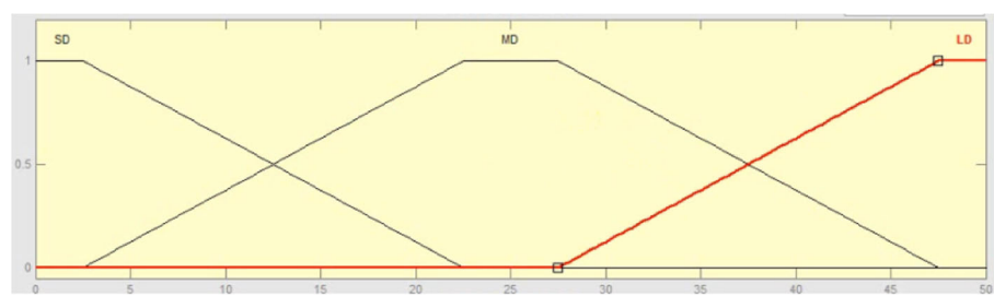
Fig. 17 Membership function of Number of Loan Repayments Past Due. The factors applied in this model as predictors are different from the previous researches. We defined these factors and a group of 10 top risk managers in several meetings approved them. Some of the factors do not change through the time, we called them certain factors. Others do, and we called them uncertain factors. We have applied fuzzy theory to uncertain factors. The fuzzy variables used to create the FIS rule base of this research were defined based on trapezoidal fuzzy numbers
