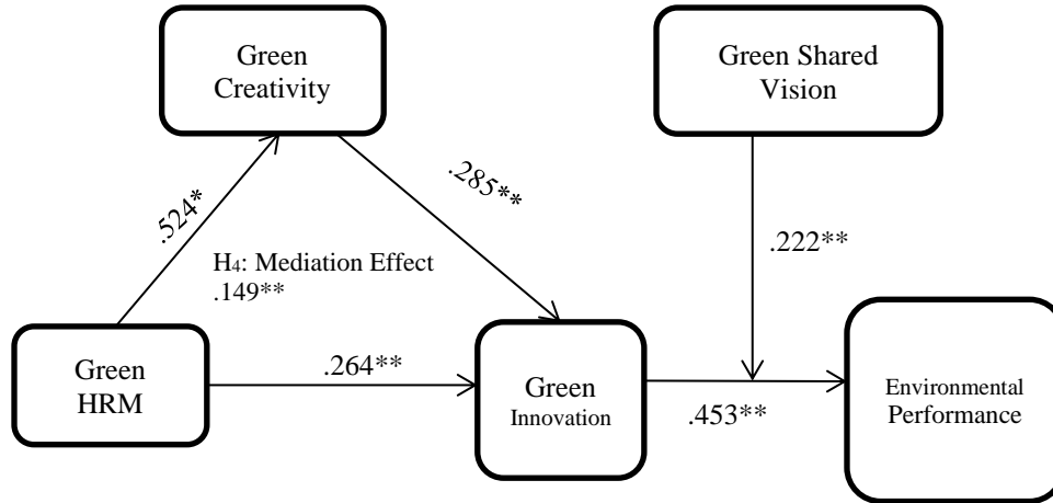
Figure 2: Structural Equation Modeling
