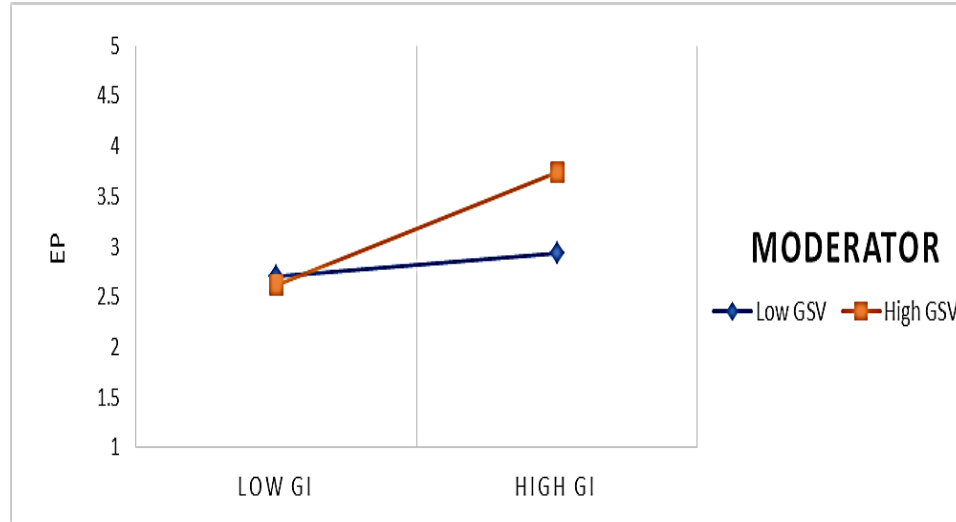
Figure 2: Moderating Effect of GSV between GI and EP
