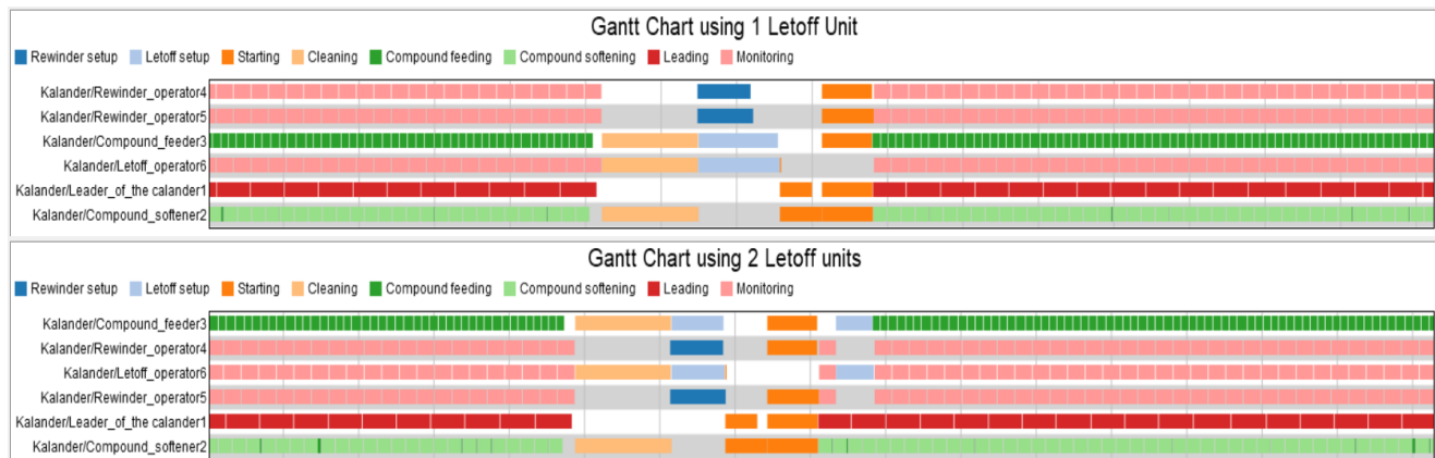
Figure 8. Gant diagram of setup times – one and two letoff units used ( Source: Own study )
