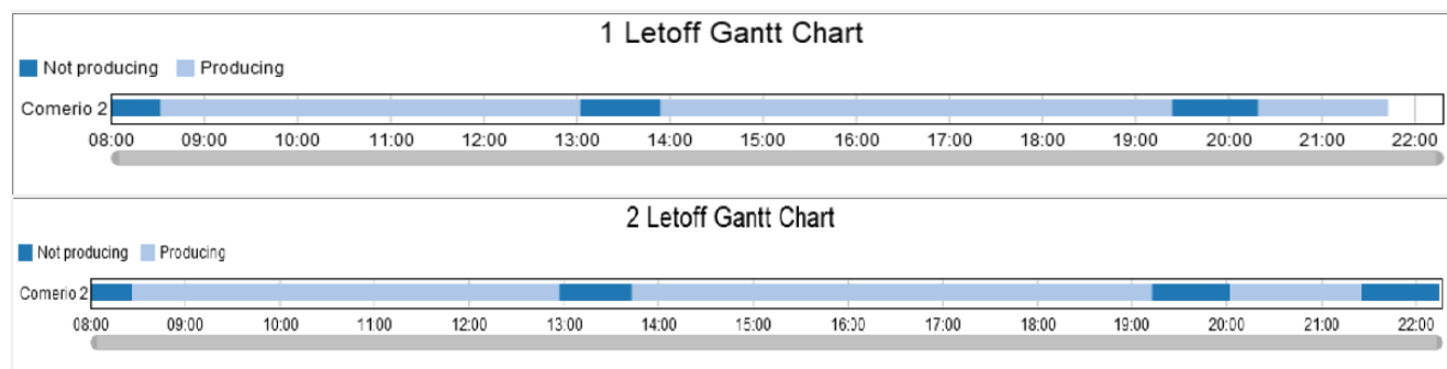
Figure 9. Gant diagram of machine downtime and process time with one and two letoff units used ( Source: Own study )
