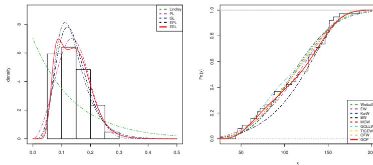
Figure 5: Fitted densities of distributions.
