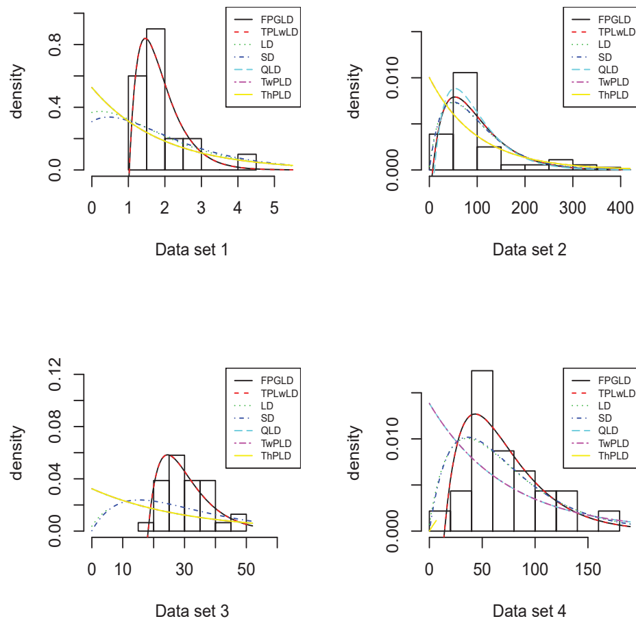
Figure 3: Empirical histograms with fitted densities of distributions
