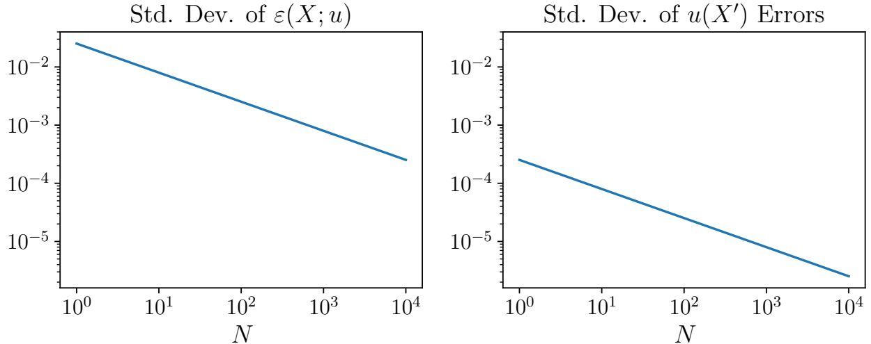
Figure 1: The concentration of Euler residuals \varepsilon(X; u) and the optimal policy u(X') for \nu = \zeta = 1 .
